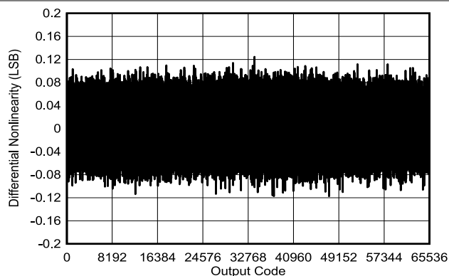
Figure 6-25. Typical DNL
