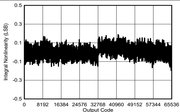
Figure 6-24. Typical INL
