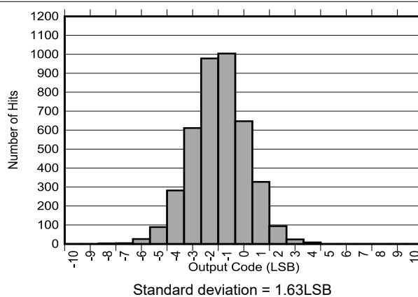
Figure 6-27. DC Input Histogram
