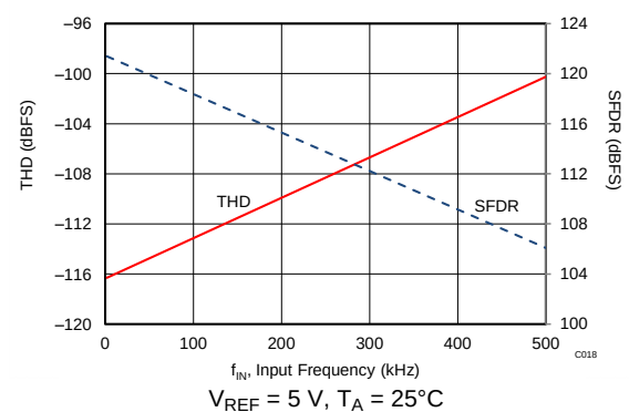
Figure 24. Distortion Performance vs Input Frequency
