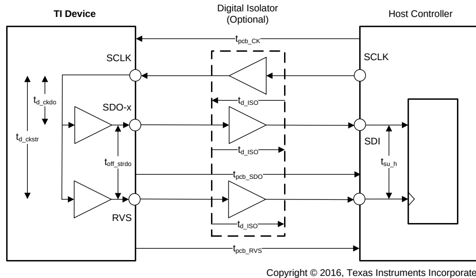
Figure 51. Delays in Source-Synchronous Communication
