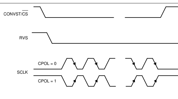
Figure 7-29. Standard SPI Timing Protocol (CPHA = 1, Single SDO-x)
