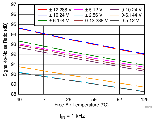
Figure 6-37. SNR vs Temperature
