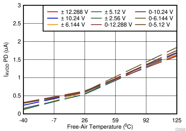
Figure 6-46. AVDD Current vs Temperature (Power-Down Mode)
