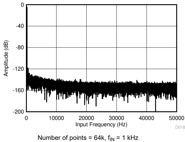
Figure 6-35. Typical FFT Plot (All Ranges) for the ADS8699
