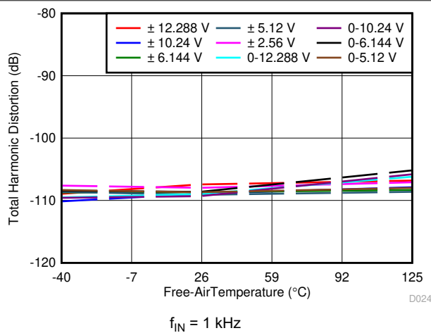
Figure 6-41. THD vs Temperature
