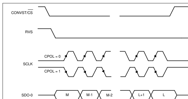
Figure 7-28. Standard SPI Timing Protocol (CPHA = 0, Single SDO-x)
