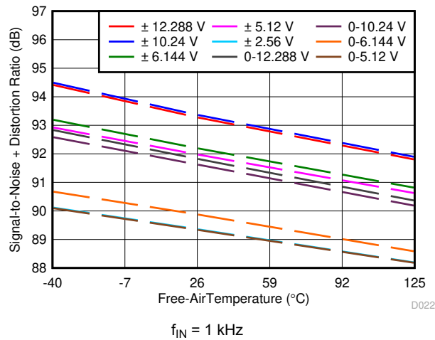
Figure 6-39. SINAD vs Temperature
