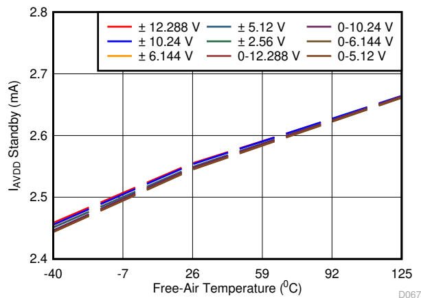
Figure 6-45. AVDD Current vs Temperature (Standby Mode)
