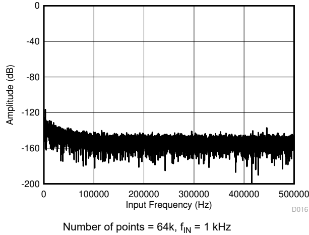
Figure 6-33. Typical FFT Plot (All Ranges) for the ADS8691
