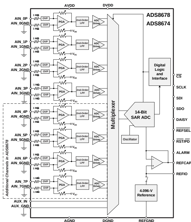
Block Diagram
