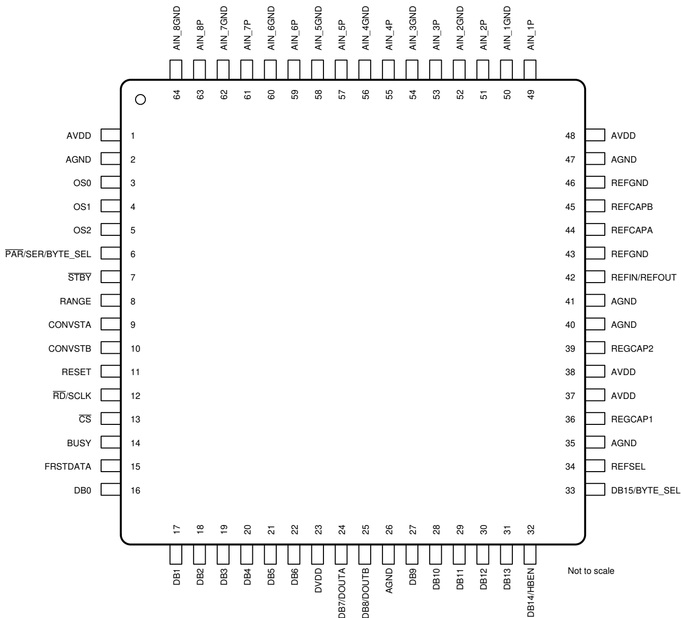
Figure 5-1. PM Package, 64-Pin LQFP (Top View)
