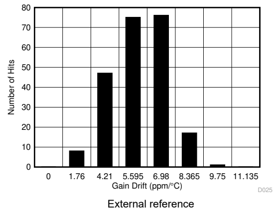
Figure 6-29. Gain Error Drift Histogram Free-Air Distribution ( \pm 5\text{ V} )
