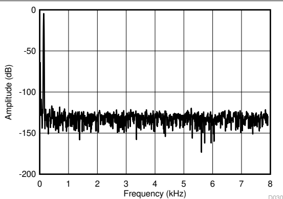
Figure 6-34. Typical FFT Plot for OSR 32x (±10 V)
