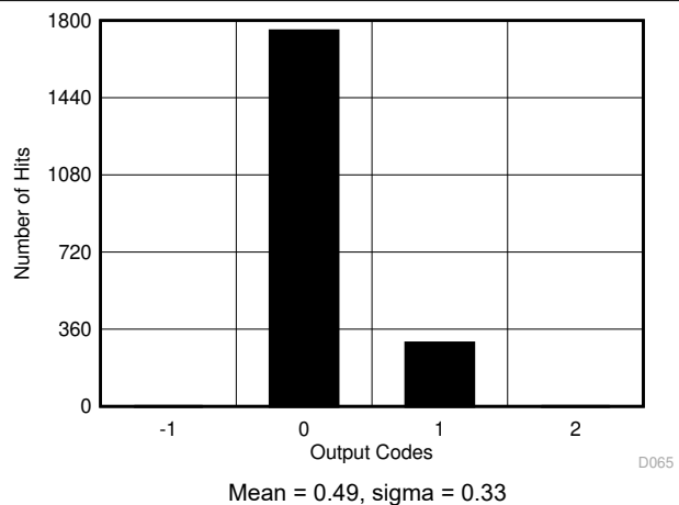
Figure 7-24. DC Histogram for OSR16
