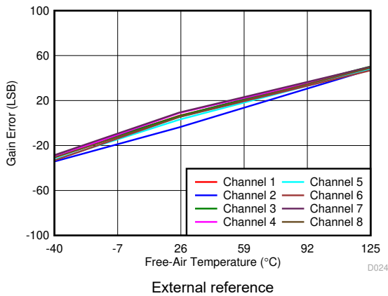
Figure 6-28. Gain Error Across Channels vs Free-Air Temperature ( \pm 10\text{ V} )
