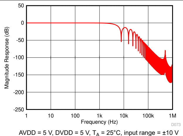
Figure 7-32. Digital Filter Response for OSR = 64
