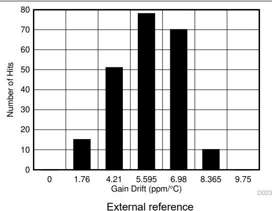
Figure 6-27. Gain Error Drift Histogram Distribution ( \pm 10\text{ V} )
