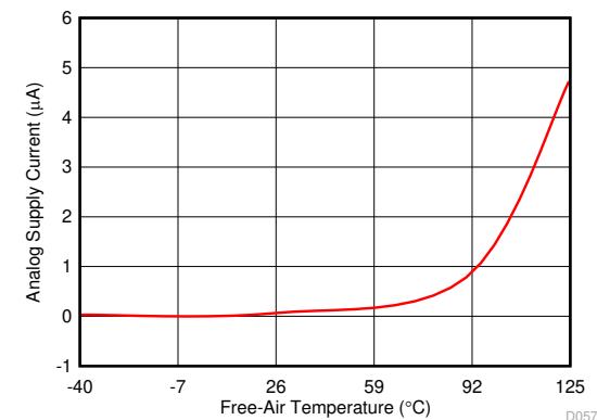
Figure 6-49. Analog Supply Current (Static) vs Free-Air Temperature (Sampling)
