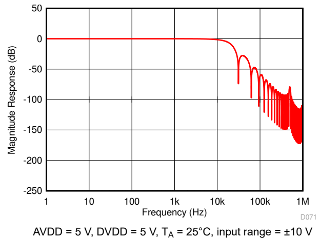
Figure 7-30. Digital Filter Response for OSR = 16
