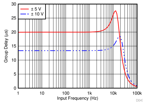
Figure 7-5. Third-Order LPF Phase Response
