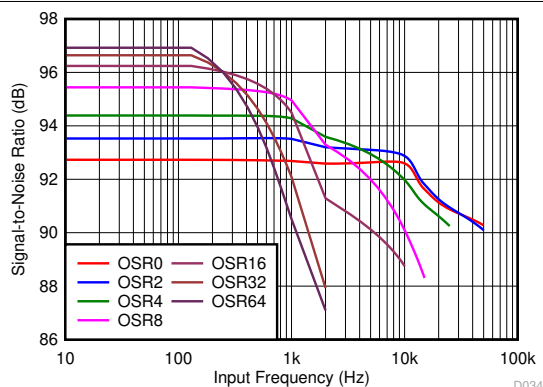
Figure 6-38. SNR vs Input Frequency for Different OSR (±10 V)
