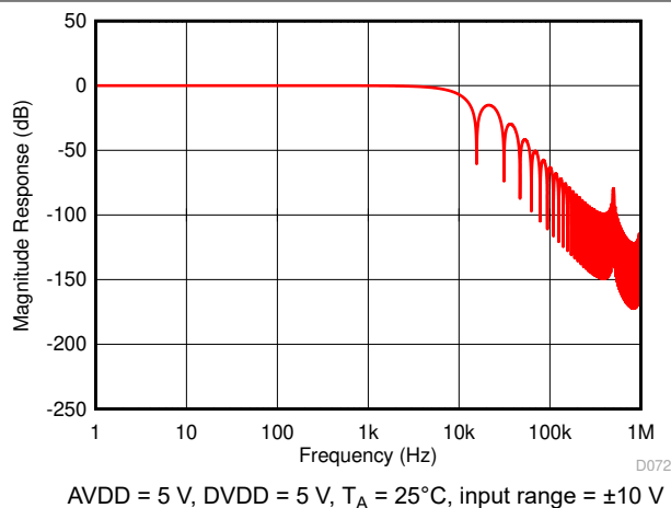
Figure 7-31. Digital Filter Response for OSR = 32
