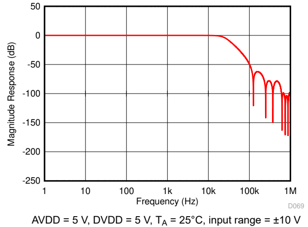
Figure 7-28. Digital Filter Response for OSR = 4
