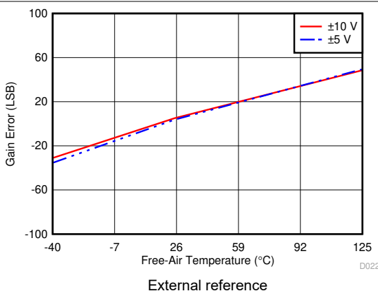
Figure 6-26. Gain Error vs Temperature
