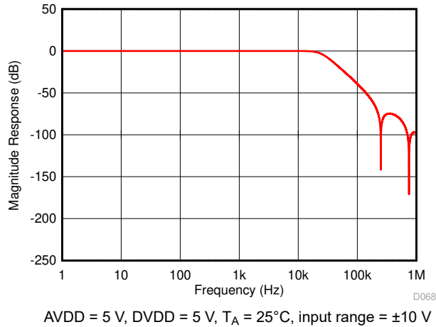
Figure 7-27. Digital Filter Response for OSR = 2
