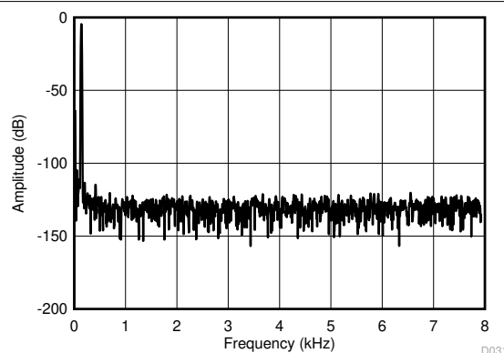
Figure 6-35. Typical FFT Plot for OSR 32x (±5 V)
