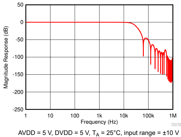
Figure 7-29. Digital Filter Response for OSR = 8
