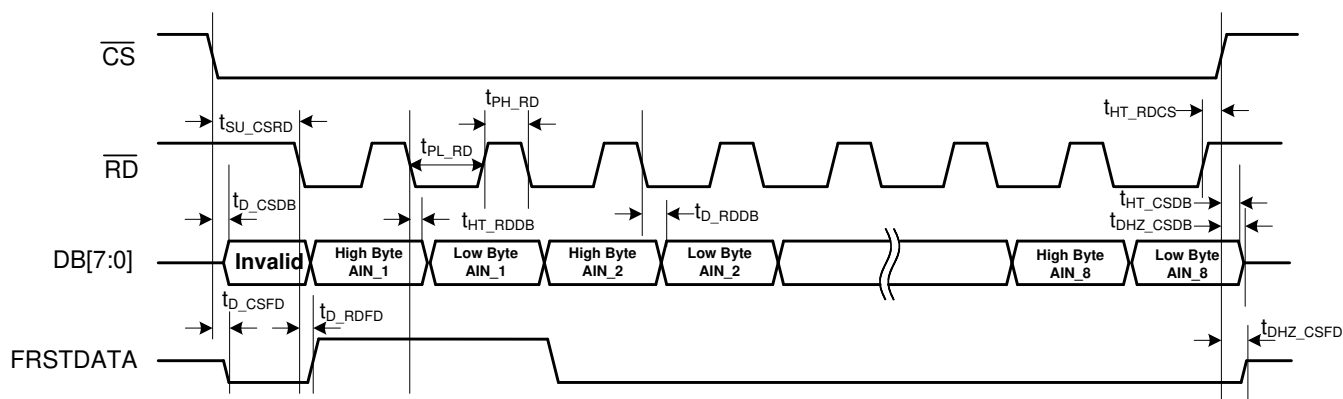
Figure 6-6. Byte Mode Data Read Operation Timing Diagram
