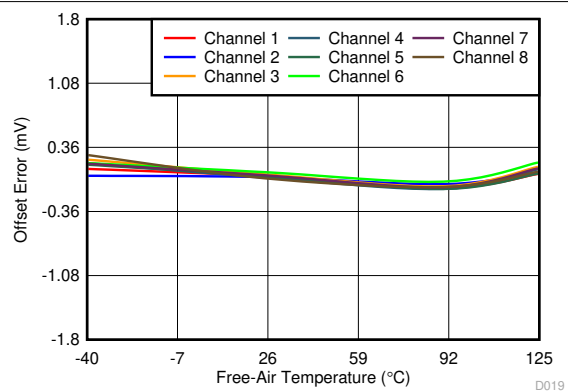
Figure 6-23. Offset Error Across Channels vs Free-Air Temperature ( \pm 10\text{ V} )
