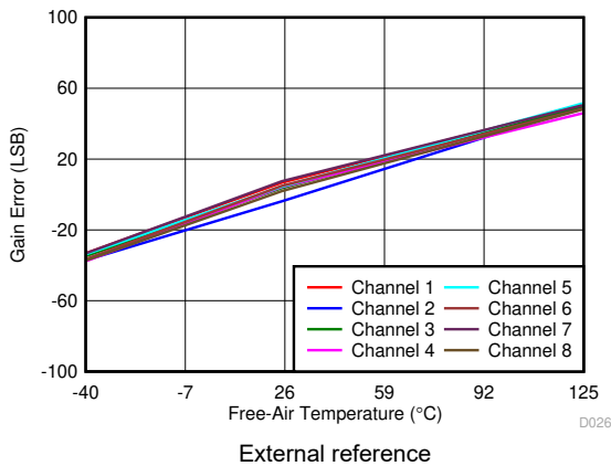
Figure 6-30. Gain Error Across Channels vs Free-Air Temperature ( \pm 5\text{ V} )
