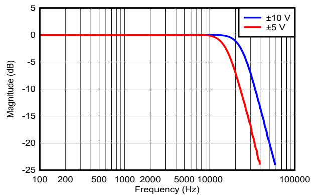
Figure 7-4. Third-Order LPF Magnitude Response
