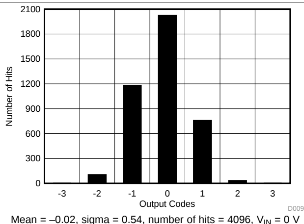
Figure 14. DC Histogram of Codes ( \pm 5\text{ V} )
