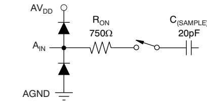
Equivalent Analog Input Circuit
