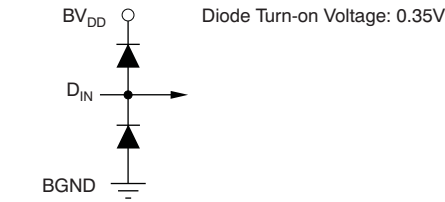
Equivalent Digital Input Circuit
