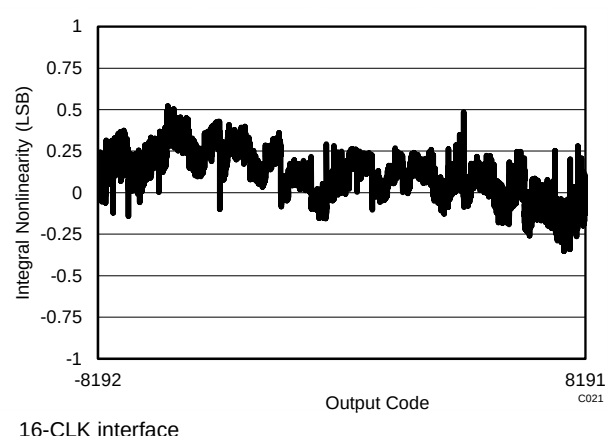
Figure 45. Typical INL
