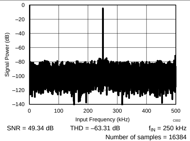
Figure 3. Typical FFT
