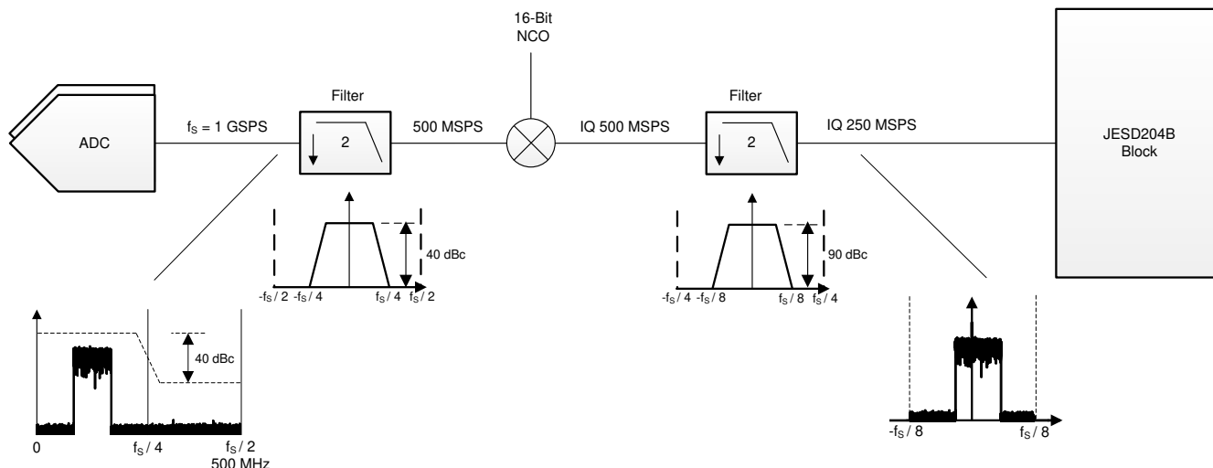
Figure 7-10. Operating Mode 1
