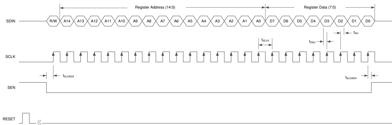
Figure 7-30. Serial Interface Write Timing Diagram
