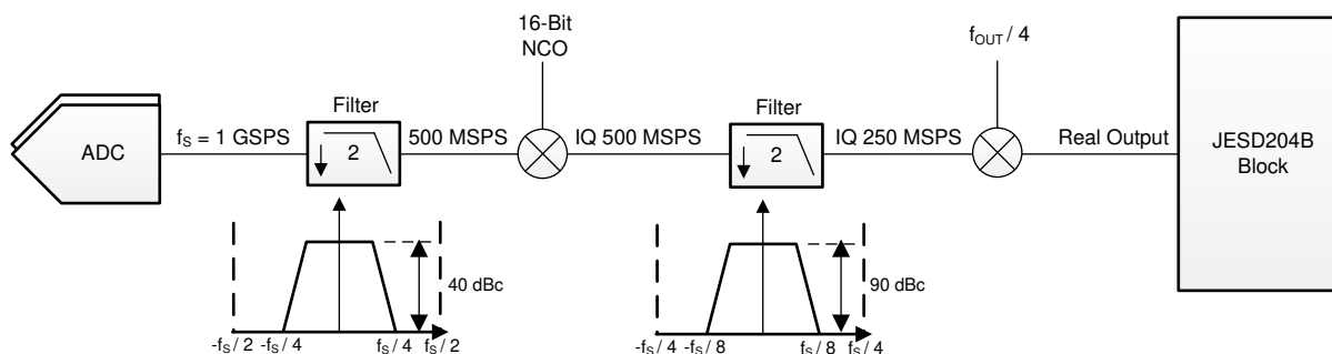
Figure 7-13. Operating Mode 4
