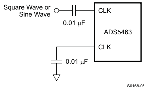
Figure 58. Single-Ended Clock
