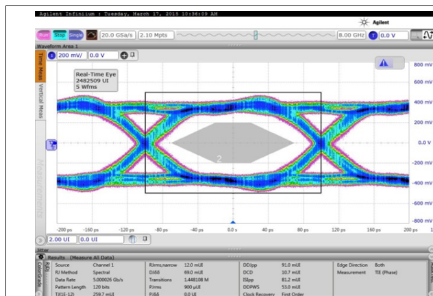
Figure 80. Eye at 5-Gbps Bit Rate with Default Output Swing
