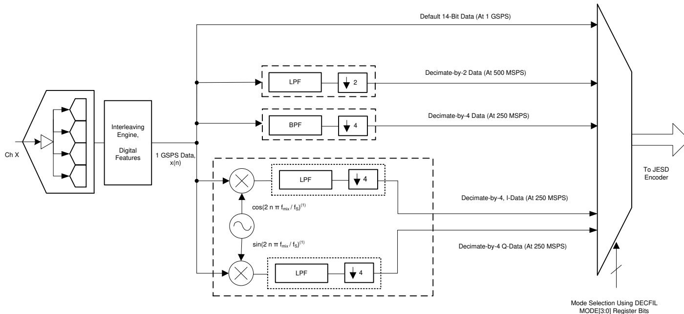
Figure 8-3. DDC Block
