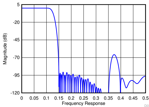
Figure 8-8. Decimate-by-4 IQ Output Filter Response
