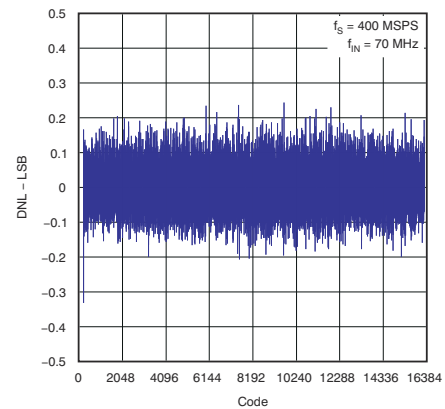
Figure 5-16. Differential Nonlinearity
