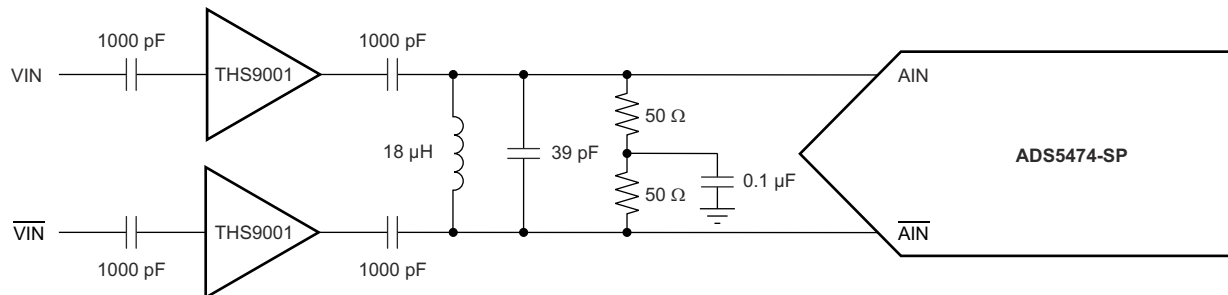
Figure 6-3. Using the THS9001 if Amplifier With the ADS5474
