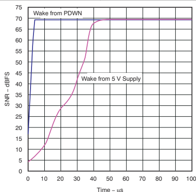
Figure 5-29. ADC Wakeup Time
