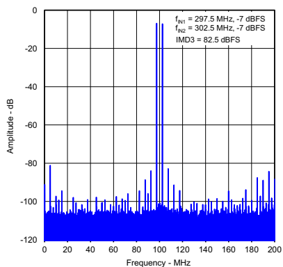
Figure 5-12. Two-Tone Intermodulation Distortion (FFT for 297.5MHz and 302.5MHz at -7\text{ dBFS} )
