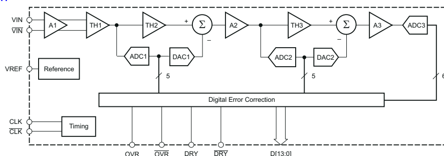
Simplified Schematic
