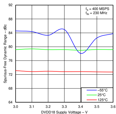
Figure 5-26. SFDR vs DVDD18 Over Temperature
