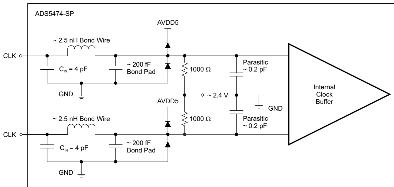
Figure 6-5. Clock Input Circuit
