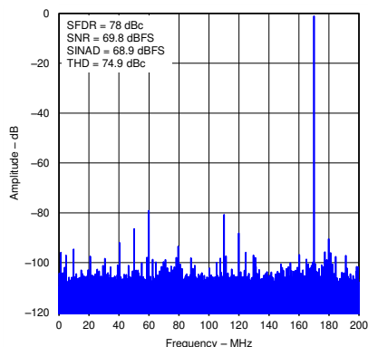
Figure 5-6. Spectral Performance FFT for 230MHz Input Signal
