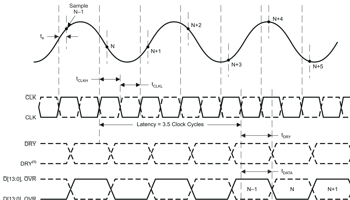
Figure 5-2. Timing Diagram
