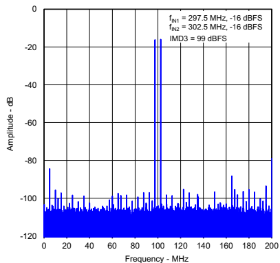
Figure 5-14. Two-Tone Intermodulation Distortion (FFT for 297.5MHz and 302.5MHz at -16\text{ dBFS} )
