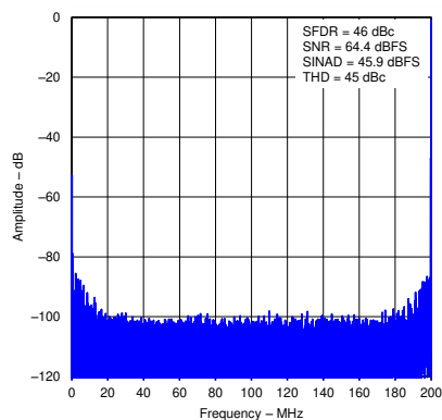
Figure 5-10. Spectral Performance FFT for 999MHz Input Signal
