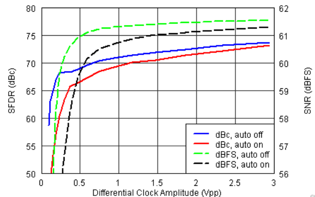
Figure 26. Performance Across Clock Amplitude
