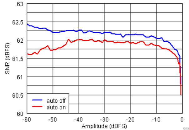
Figure 16. SNR vs Amplitude ( f_{\text{in}} = 230\text{ MHz} )
