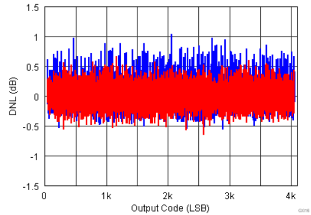
Figure 28. DNL
