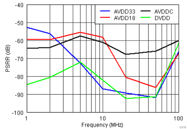
Figure 30. PSRR Across Frequency
