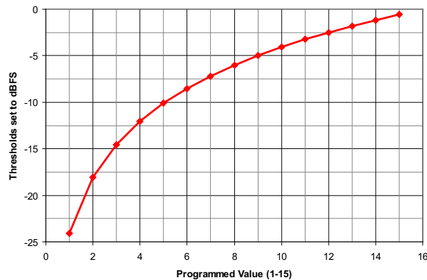
Figure 51. OVR Detection Threshold
