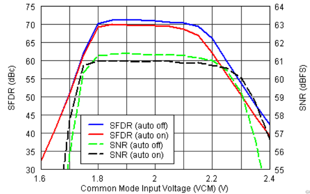
Figure 22. Performance Across Input Common-Mode Voltage ( f_{\text{in}} = 230 \text{ MHz} )
