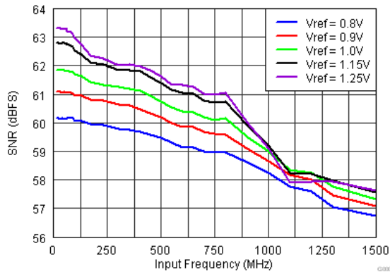
Figure 21. SNR vs Vref (Auto Off)
