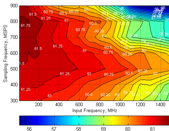
Figure 35. SNR Across Input and Sampling Frequencies (Auto On)
