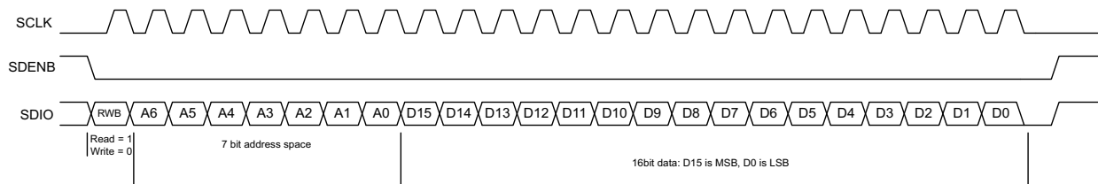
Figure 47. Serial Register Read Timing Diagram
