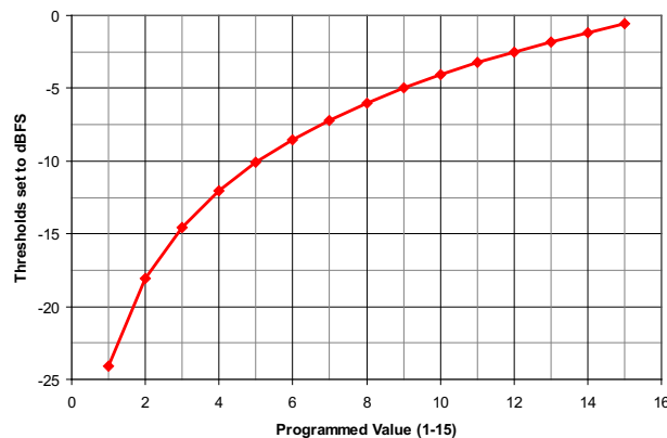
Figure 38. OVR Detection Threshold
