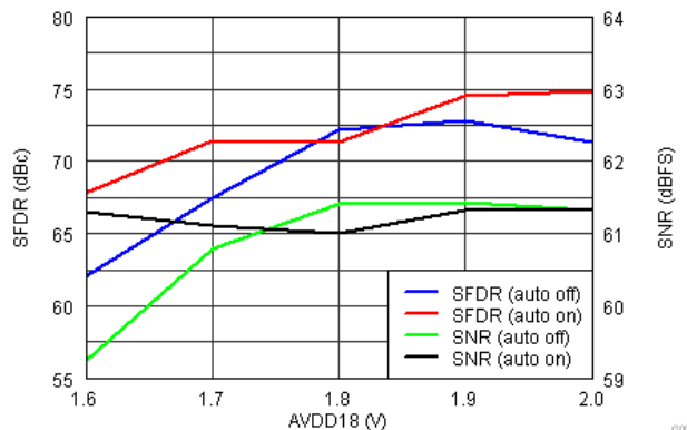
Figure 25. Performance Across AVDD18 ( f_{\text{in}} = 230\text{MHz} )
