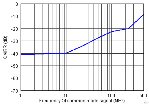
Figure 29. CMRR Across Frequency
