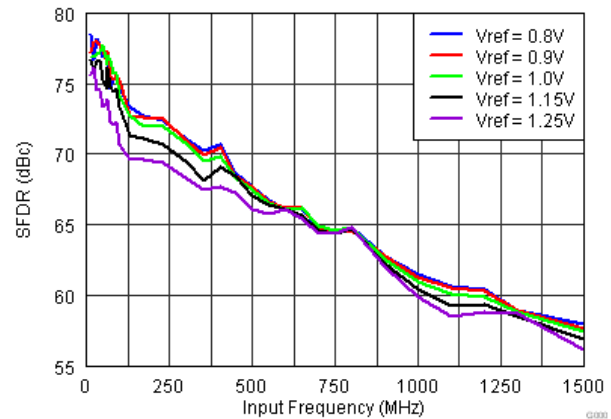
Figure 18. SFDR vs Vref (Auto On)
