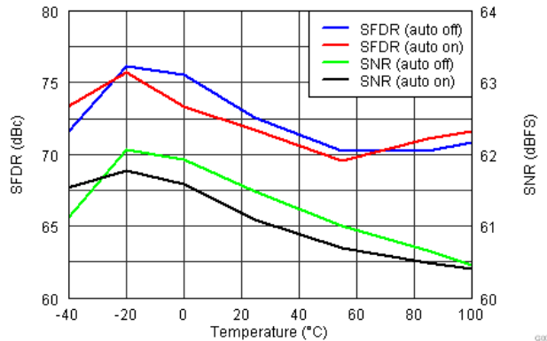
Figure 23. Performance Across Temperature ( f_{\text{in}} = 230 \text{ MHz} )
