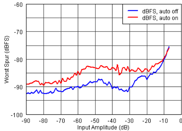
Figure 17. Tow Tone Performance Across Input Amplitude ( f_{\text{in}} = 170\text{ MHz} )
