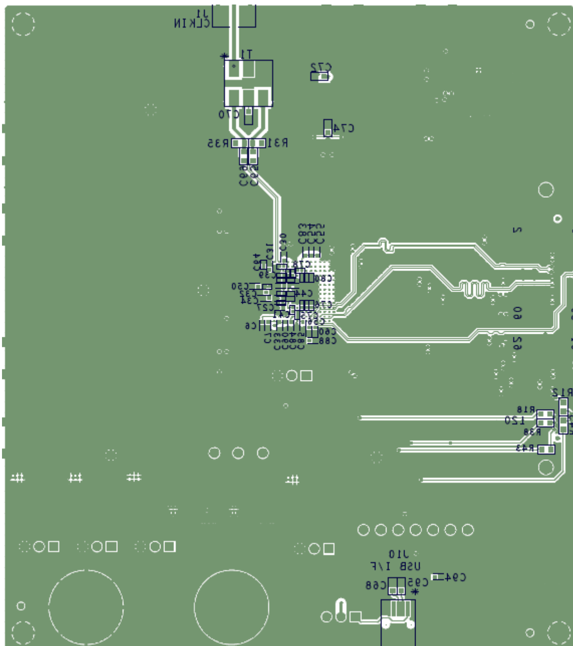
Figure 66. Bottom Layer
