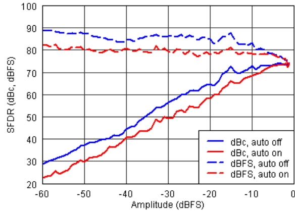
Figure 15. SFDR vs Amplitude ( f_{\text{in}} = 230\text{ MHz} )
