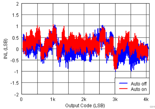
Figure 27. INL
