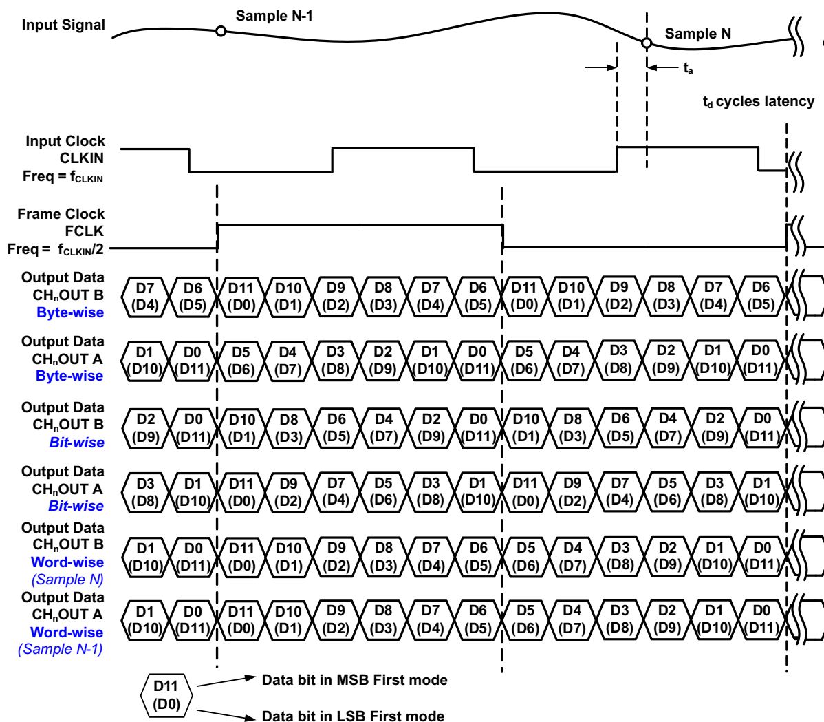
Figure 53. 12-Bit Word Wise
