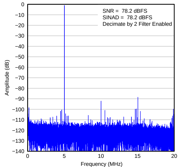
Figure 67. SNR With Decimation Enabled
