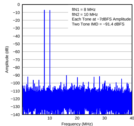
Figure 13. Two-Tone Intermodulation
