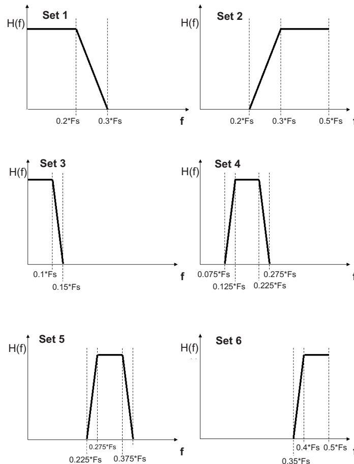
Figure 56. Filter Types
