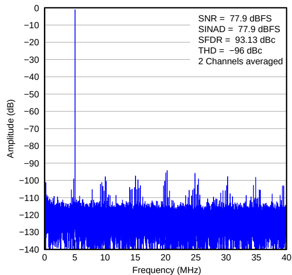
Figure 66. SNR without Decimation Enabled
