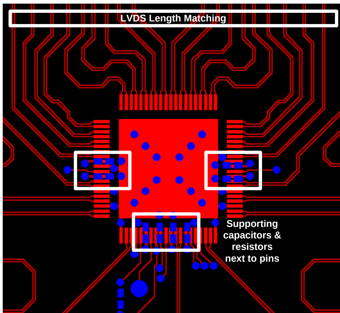
Figure 69. Layout Recommendations
