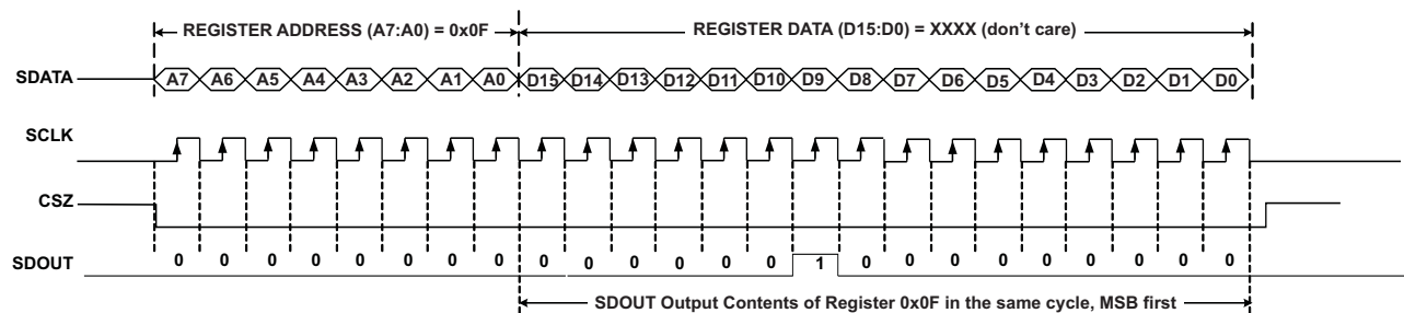
Figure 52. Serial Readout Timing
