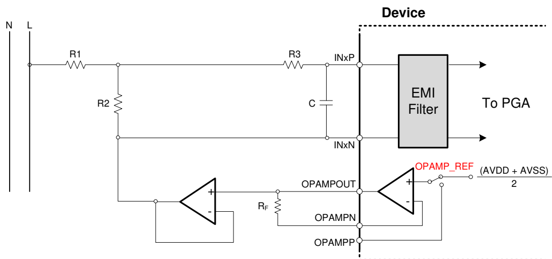
Figure 59. Simplified Voltage-Sensing Connections
