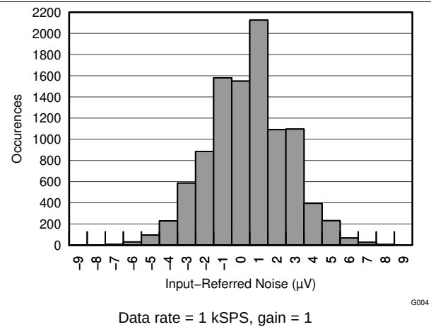
Figure 4. Noise Histogram
