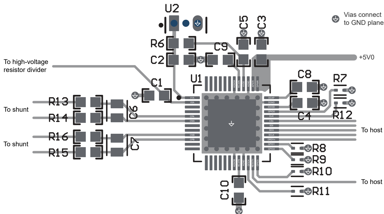
Figure 9-8. Layout Example
