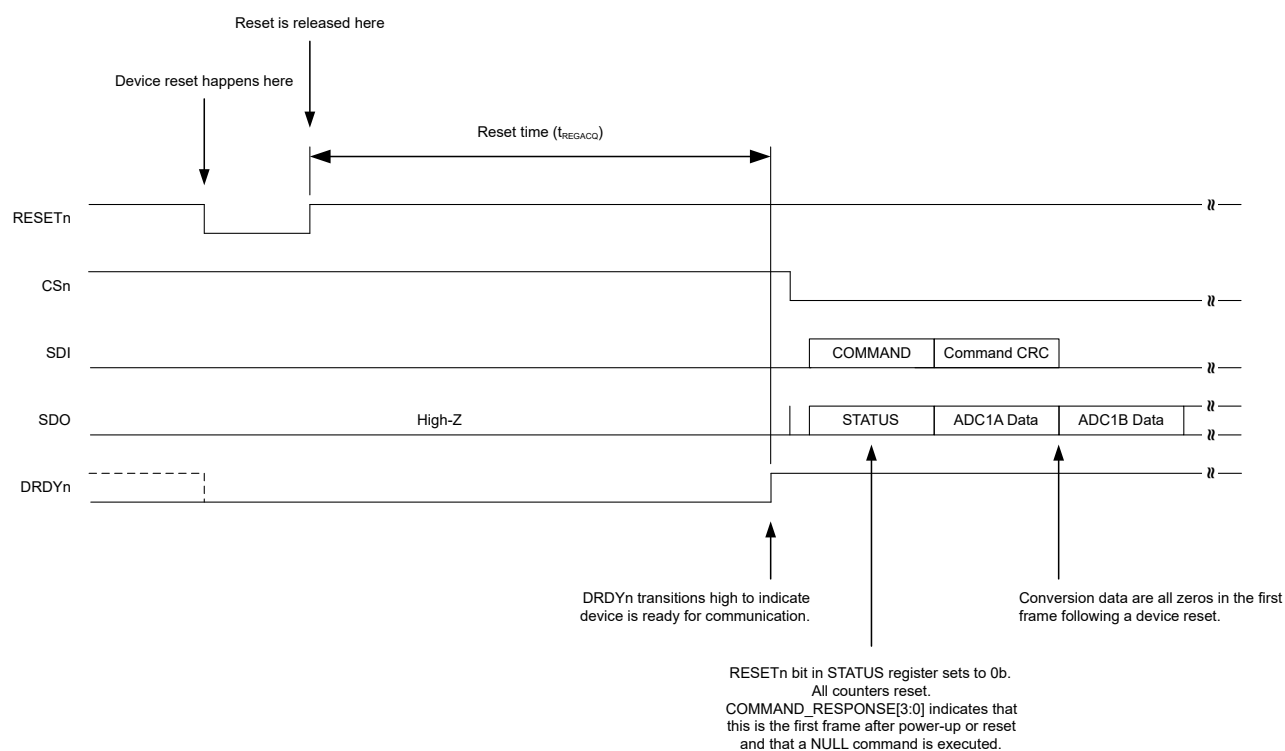
Figure 7-27. DRDYn Pin Behavior After Device Reset
