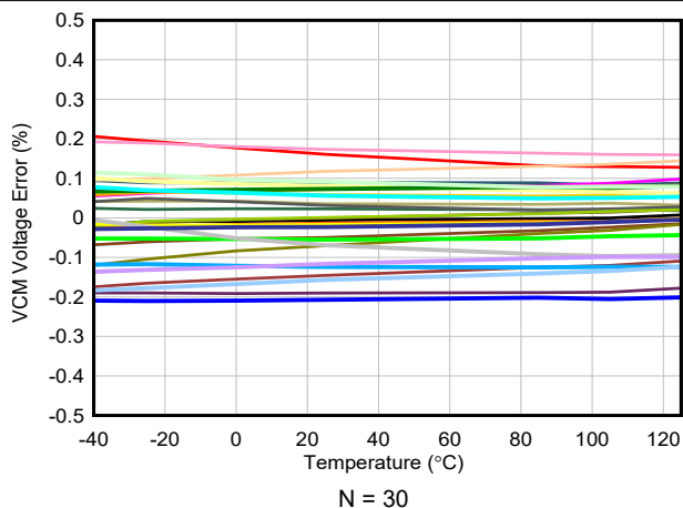
Figure 6-55. VCM Voltage vs Temperature
