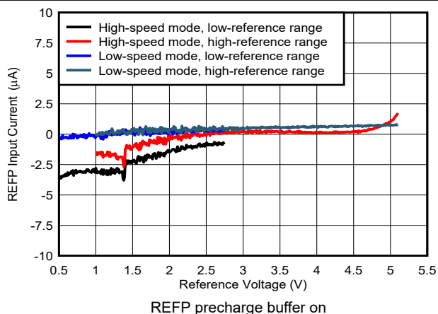
Figure 6-57. REFP Input Current vs Reference Voltage
