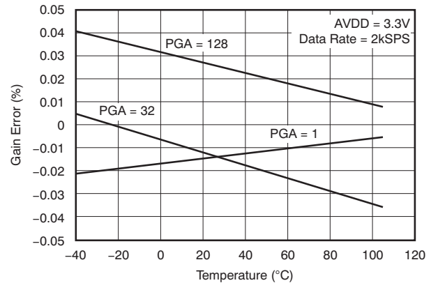
Figure 24. Gain Error vs Temperature
