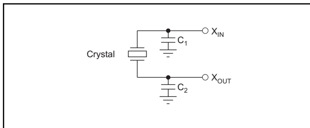
Figure 6. Crystal Connection.
