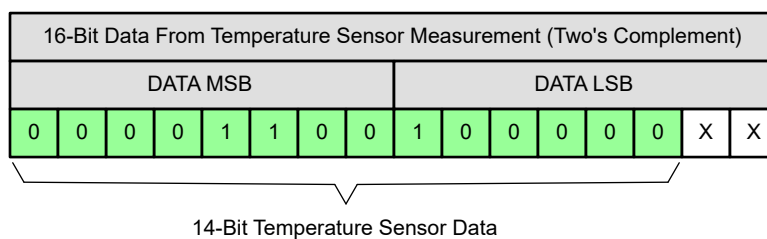
Figure 8-23. 14-Bit Temperature Sensor Data Alignment Within 16-Bit Conversion Result
