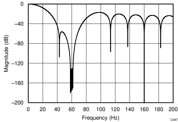
Figure 8-13. Filter Response (DR = 20SPS)
