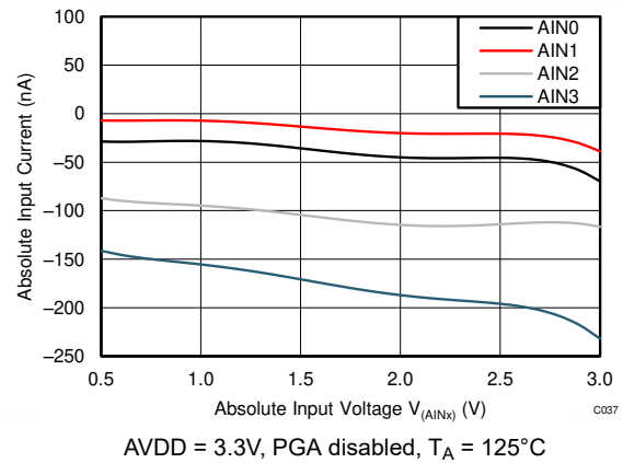
Figure 6-24. Absolute Input Current vs Absolute Input Voltage
