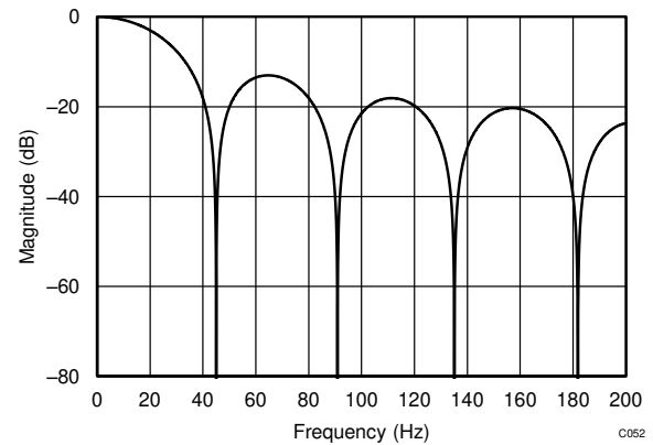
Figure 8-16. Filter Response (DR = 45SPS)
