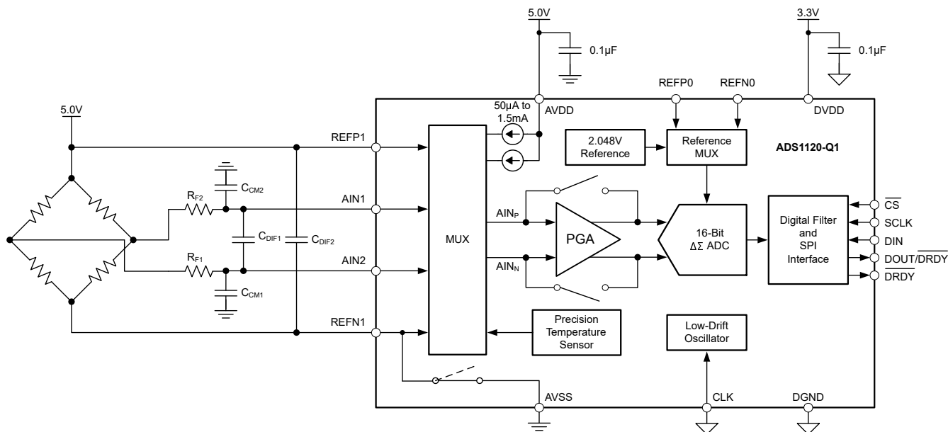
Figure 9-11. Bridge Measurement
