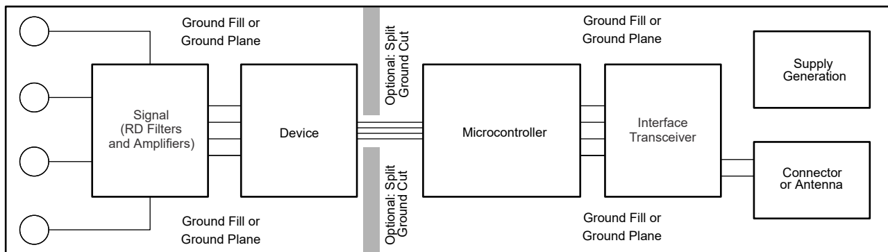
Figure 9-15. System Component Placement
