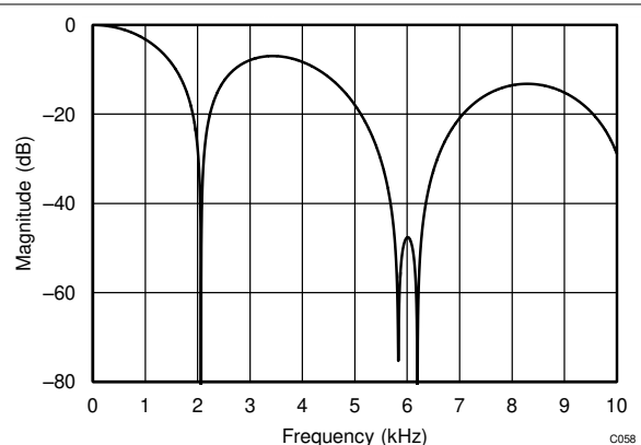
Figure 8-22. Filter Response (DR = 2kSPS)
