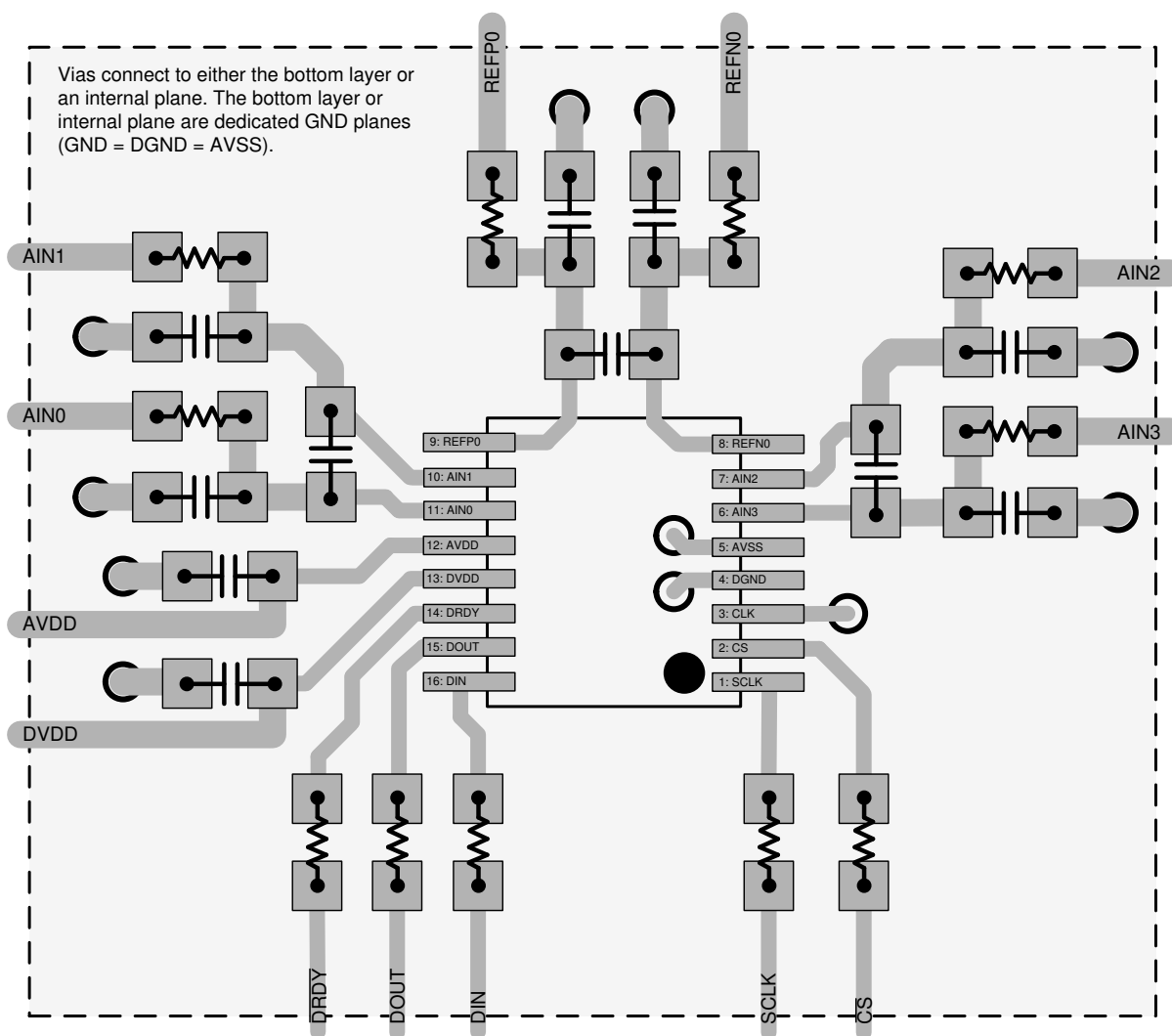
Figure 9-16. Layout Example
