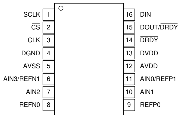
Figure 5-1. PW Package, 16-Pin TSSOP
