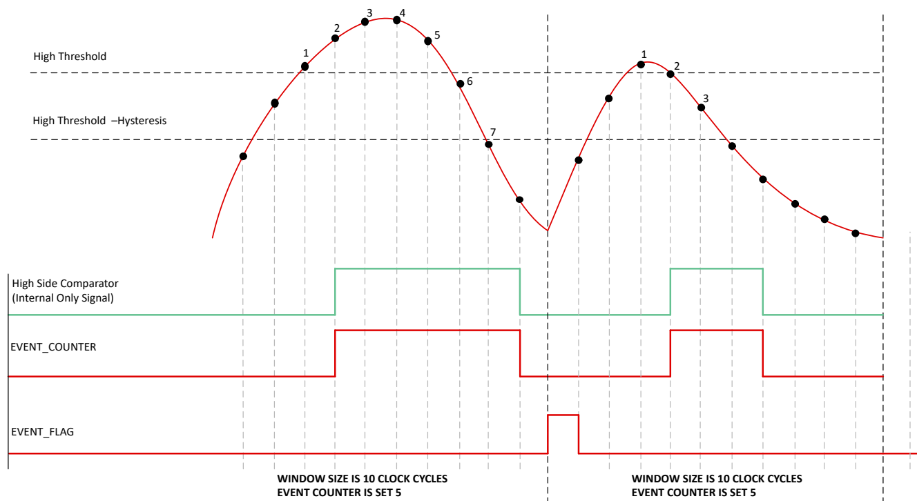
Figure 6-28. Window Monitoring
