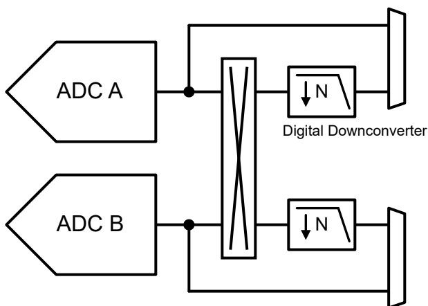
Figure 6-10. Digital down converter data multiplexer
