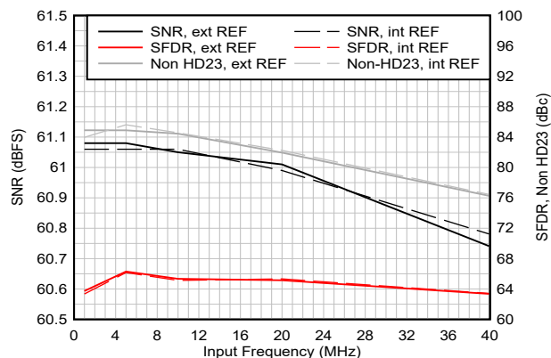
Figure 5-10. AC Performance vs Input Frequency
