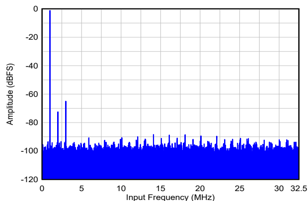
Figure 5-24. Single Tone FFT at F_{IN} = 1\text{MHz}
