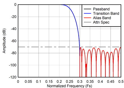
Figure 6-12. Decimation by 2 frequency response
