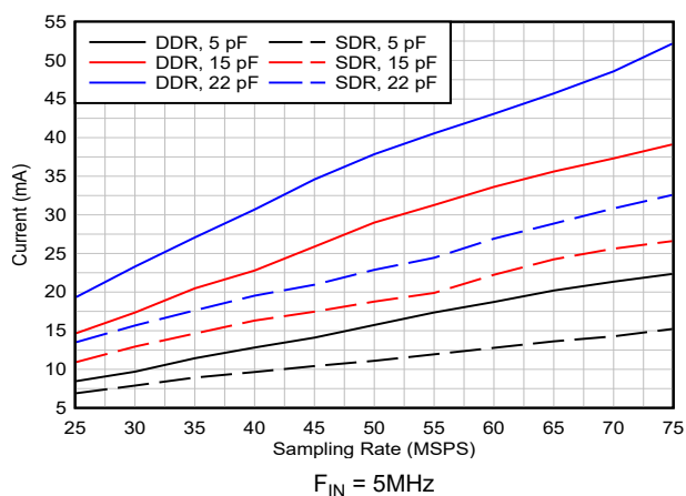
Figure 5-43. I_{OVDD} Current vs Load Capacitance
