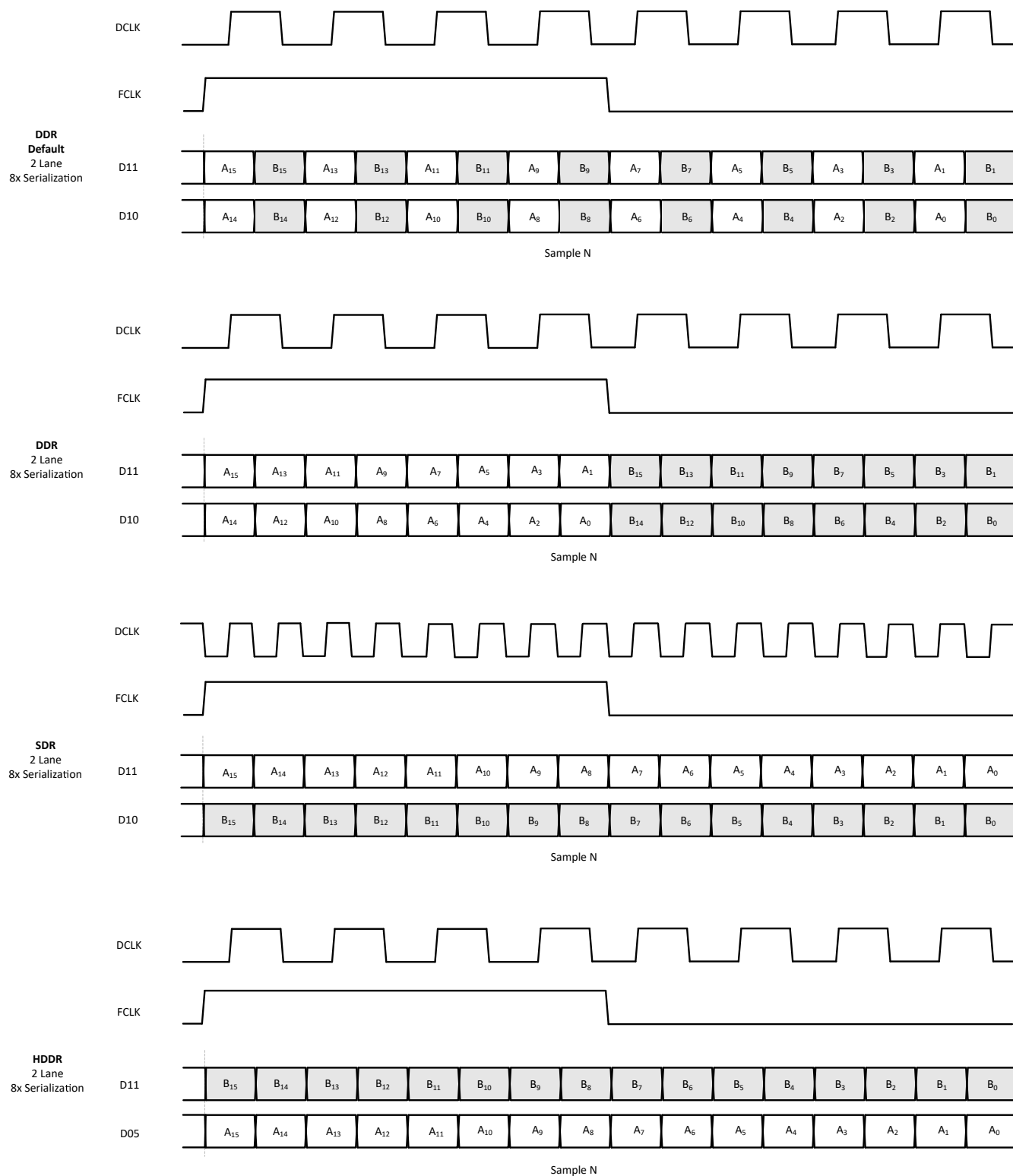
Figure 6-23. 16 Bit, 2 Lanes, 8x Serialization
