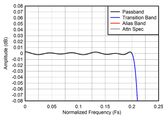
Figure 6-13. Decimation by 2 passband ripple response
