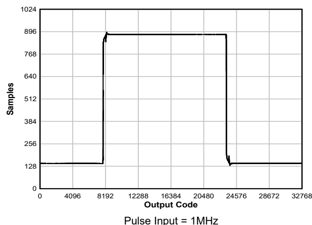
Figure 5-19. Pulse Response
