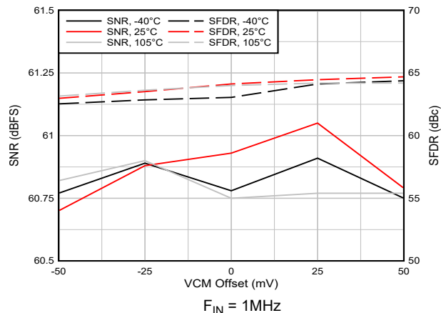
Figure 5-15. AC Performance vs VCM vs Temperature
