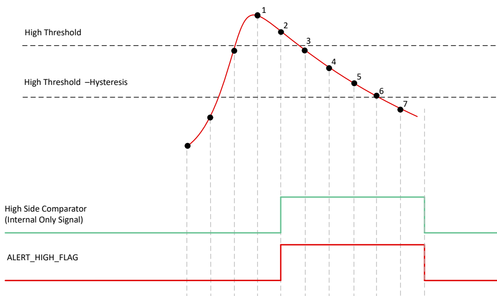
Figure 6-27. Event Monitoring
