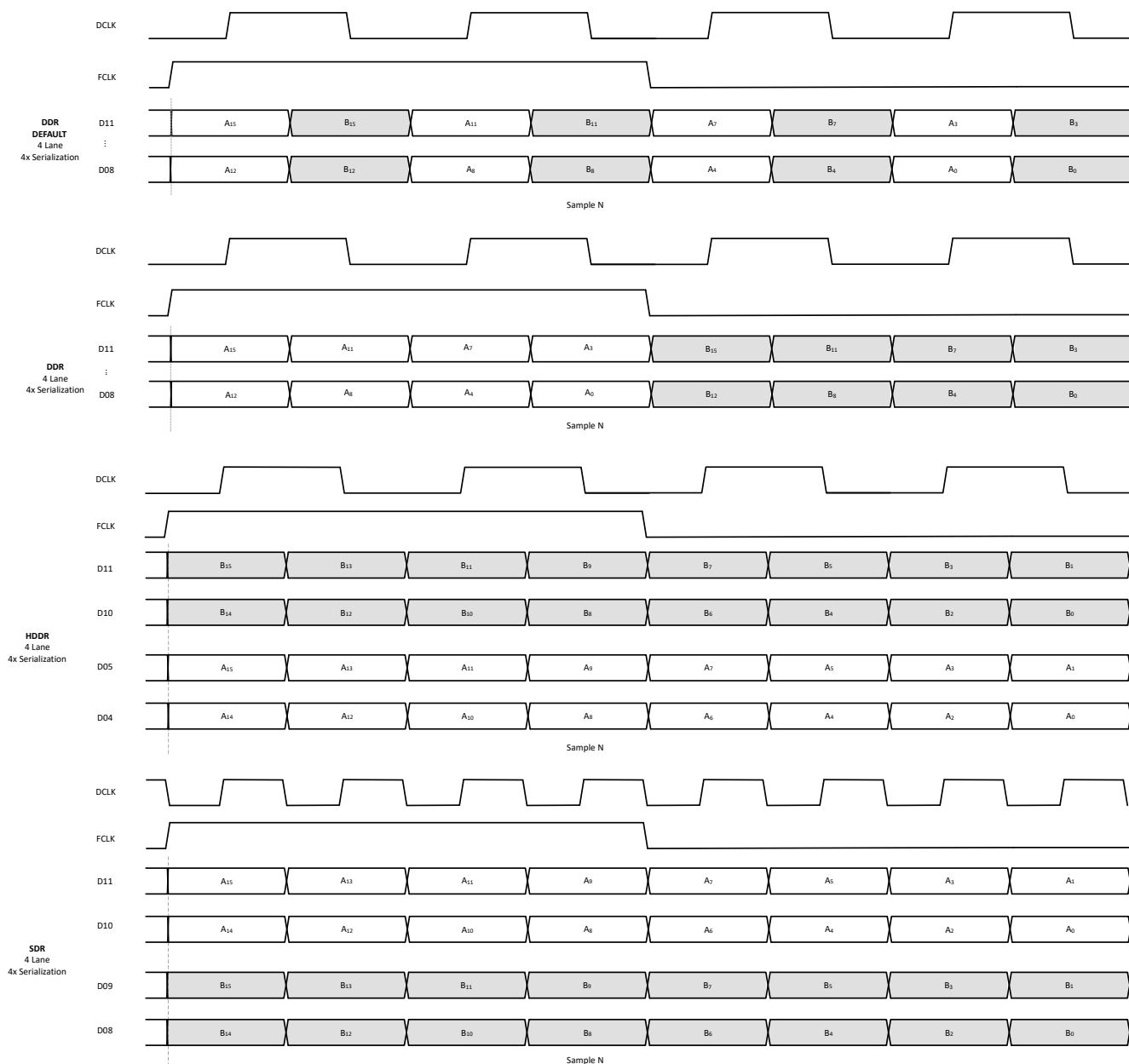
Figure 6-22. 16 Bit, 4 Lanes, 4x Serialization
