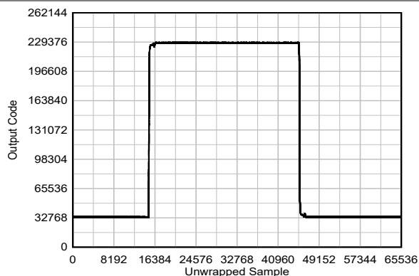
Unwrapped 1MHz Square Wave Figure 5-20. Pulse Response
