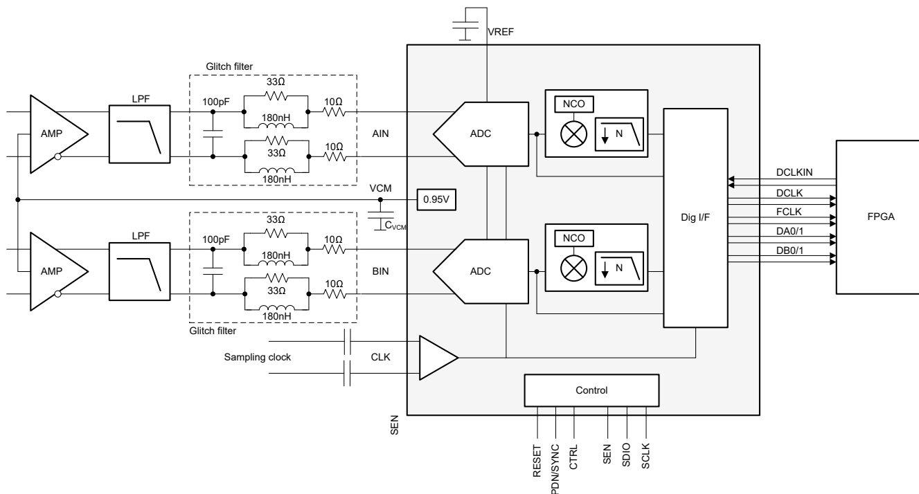
Figure 8-1. Typical Configuration of a DC Coupled Digitizer
