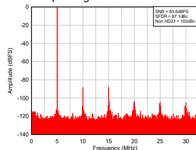
Single Tone Spectrum, F_s = 65 MSPS, F_{in} = 5 MHz
