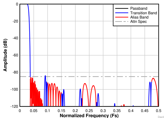
Figure 7-27. Decimation by 16 Filter Frequency Response
