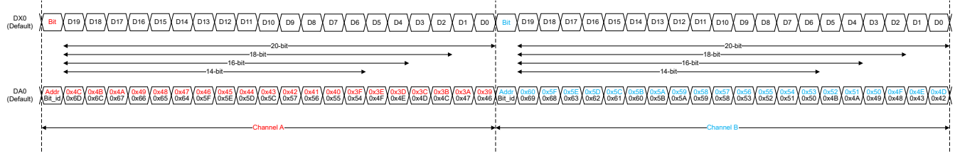
Figure 7-17. Default Bit Mapping for 1/2-wire
