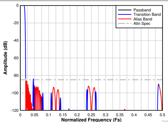
Figure 7-29. Decimation by 32 Filter Frequency Response
