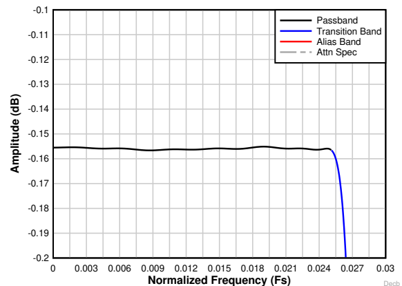
Figure 7-28. Decimation by 16 Filter Passband Ripple Response
