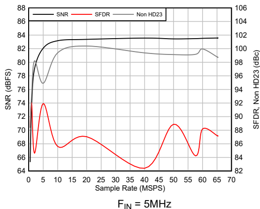
Figure 5-13. AC Performance Vs Sampling Rate
