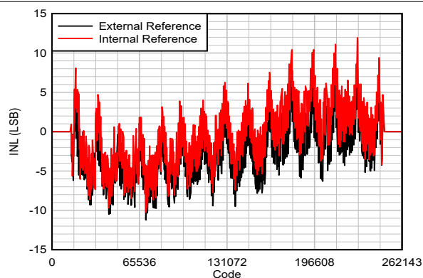
Figure 5-17. INL Vs Code
