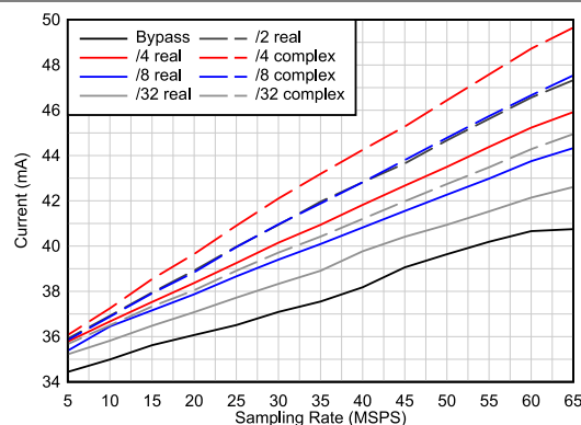
Figure 5-26. I_{OVDD} Current vs Decimation
