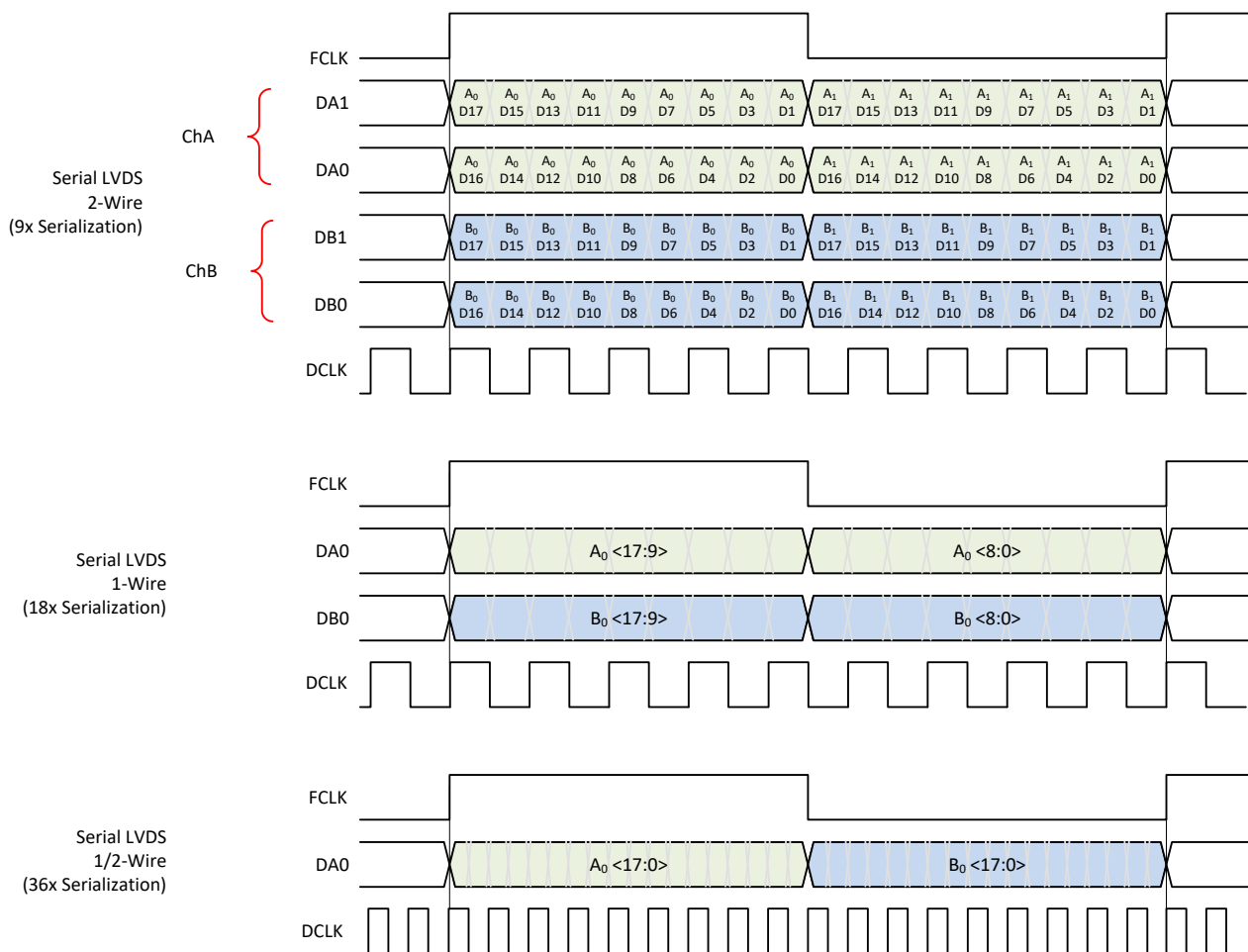
Figure 8-39. Output Data Format in Real Decimation (18-bit Output Resolution)
