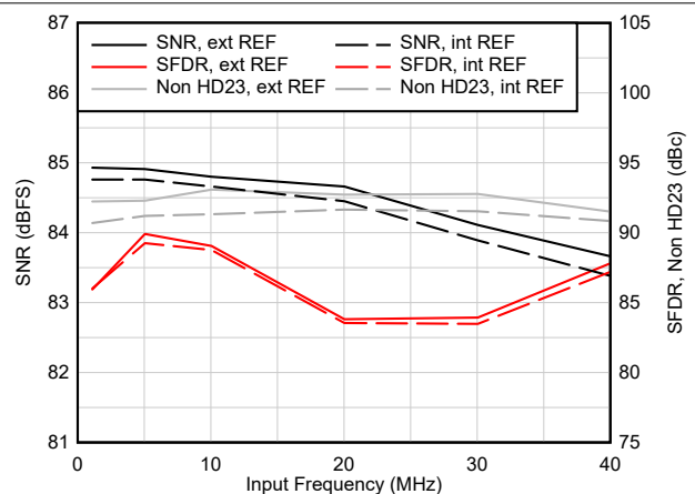
Figure 6-27. AC Performance vs Input Frequency
