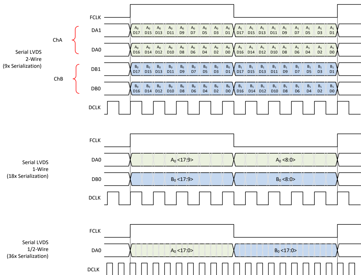
Figure 8-40. Output Data Format in Real Decimation (18-bit Output Resolution)
