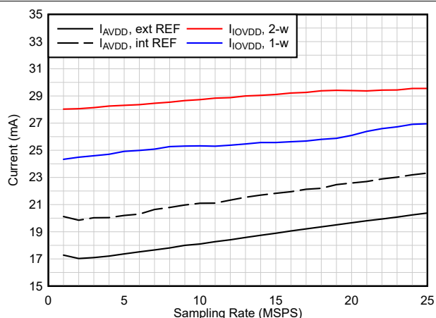
Figure 6-37. Current vs Sampling Rate F_{IN} = 1.1 MHz, DDC Bypass
