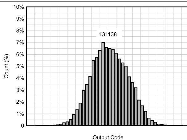
Figure 6-61. DC Histogram
