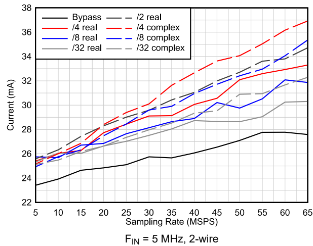
Figure 6-64. IOVDD Current vs Decimation
