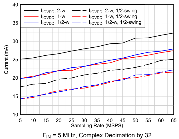
Figure 6-65. IOVDD Current vs Output Interface
