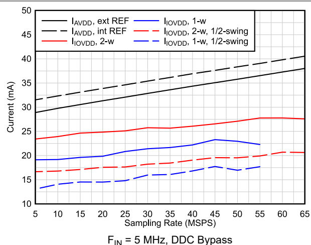
Figure 6-63. Current vs Sampling Rate
