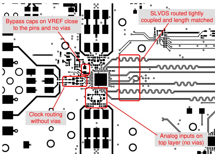
Figure 9-10. Layout example: top layer of ADC358x/368x EVM
