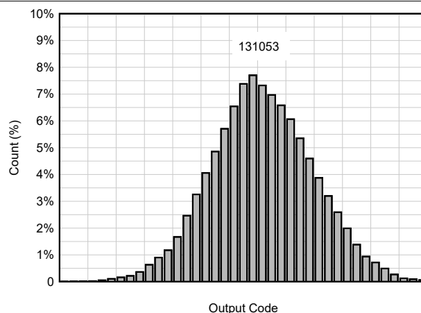
Figure 6-14. DC Offset Histogram
