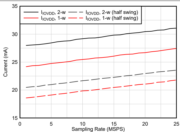
Figure 6-39. I_{IOVDD} Current vs Interface F_{IN} = 1.1 MHz, Complex Decimation by 32
