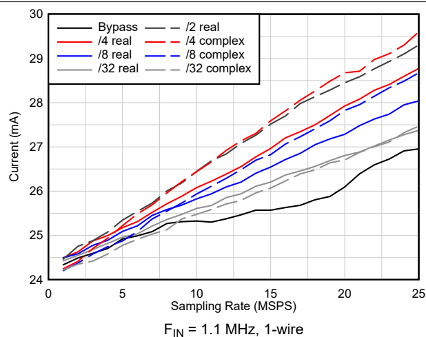
Figure 6-38. I_{IOVDD} Current vs Decimation F_{IN} = 1.1 MHz, 1-wire
