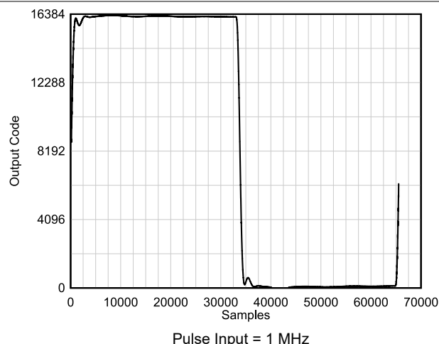
Figure 6-20. Pulse Response
