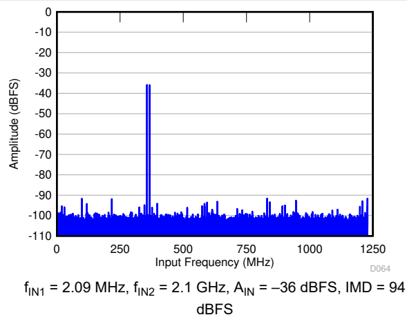
Figure 6-26. FFT for Two-Tone Input Signal (–36 dBFS, f_s = 2457.6 \text{ MSPS} )
