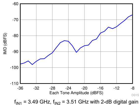
Figure 6-35. Intermodulation Distortion vs. Input Amplitude (3490 MHz and 3510 MHz)
