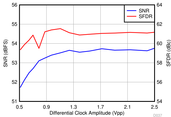
Figure 6-59. Performance vs. Amplitude
