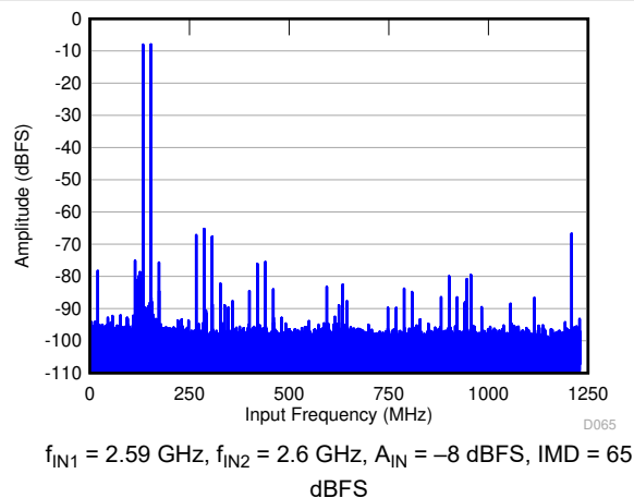
Figure 6-29. FFT for Two-Tone Input Signal (-8 dBFS, f_s = 2457.6 \text{ MSPS} )
