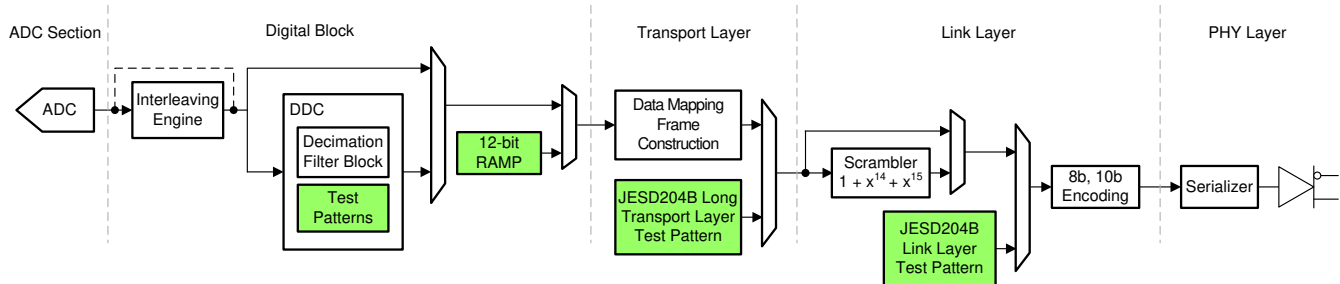
Figure 8-52. Test Pattern Generator Implementation
