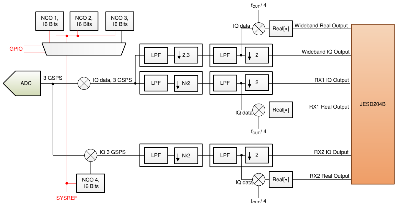
Figure 8-14. DDC Chains Overview (One ADC Channel Shown)
