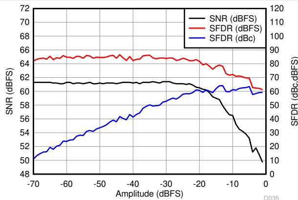
Figure 6-59. Performance vs. Amplitude
