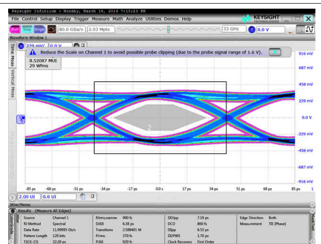
Figure 8-45. Data Eye at 12 Gbps
