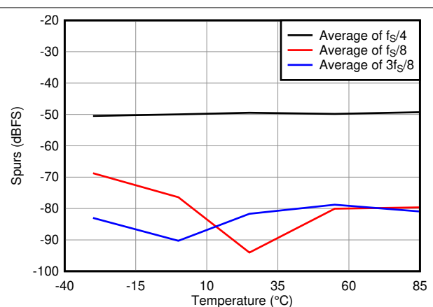
Figure 9-8. Offset Corrector Block Disabled
