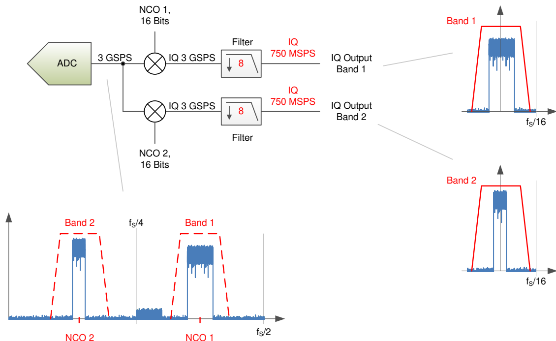
Figure 8-17. Dual-Band Example
