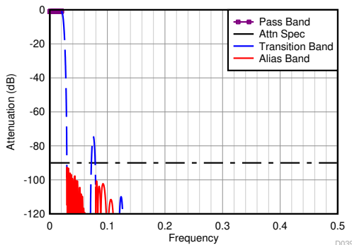
Figure 8-35. Divide-by-20 Filter Response
