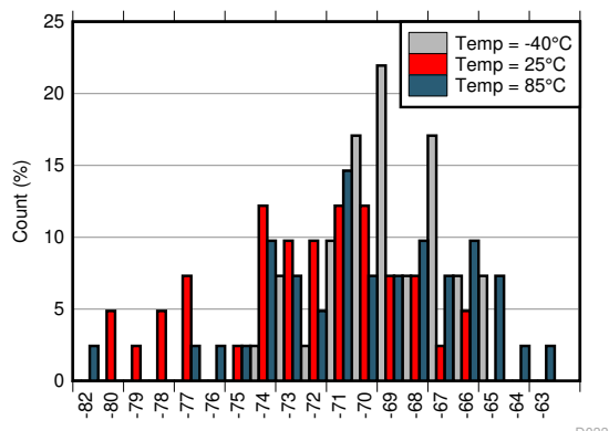
Figure 6-55. HD2 Histogram at AVDD19 = 1.8 V
