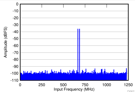
Figure 6-22. FFT for Two-Tone Input Signal (–36 dBFS, f_s = 2457.6 \text{ MSPS} )
