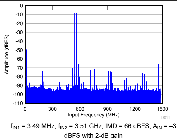
Figure 6-27. FFT for Two-Tone Input Signal (–8 dBFS)
