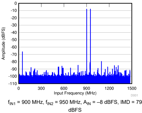
Figure 6-15. FFT for Two-Tone Input Signal (–8 dBFS)
