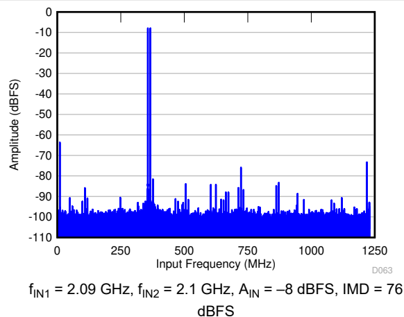
Figure 6-25. FFT for Two-Tone Input Signal (–8 dBFS, f_s = 2457.6 \text{ MSPS} )
