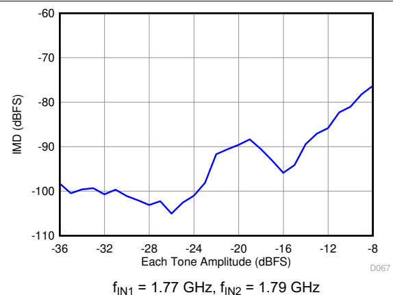
Figure 6-32. Intermodulation Distortion vs. Input Amplitude (1770 MHz and 1790 MHz, f_s = 2457.6 \text{ MSPS} )
