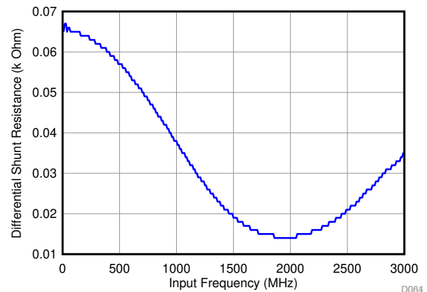
Figure 8-4. Differential Input Resistance vs. Input Frequency
