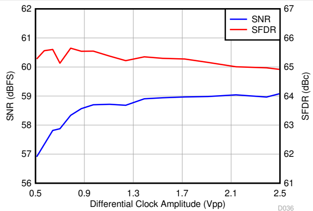
Figure 6-60. Performance vs. Clock Amplitude
