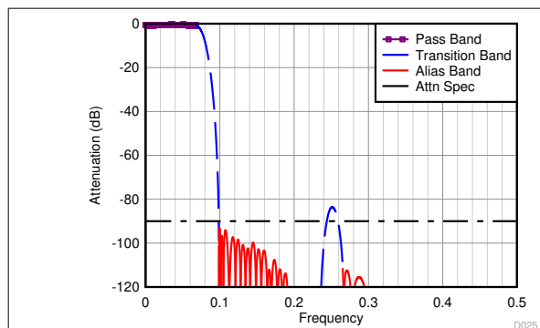
Figure 8-21. Divide-by-6 Filter Response
