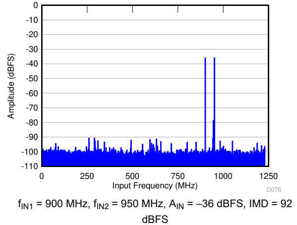
Figure 6-18. FFT for Two-Tone Input Signal (–36 dBFS, f_s = 2457.6 \text{ MSPS} )
