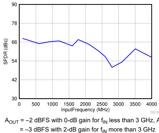
Figure 6-37. Spurious-Free Dynamic Range vs. Input Frequency
