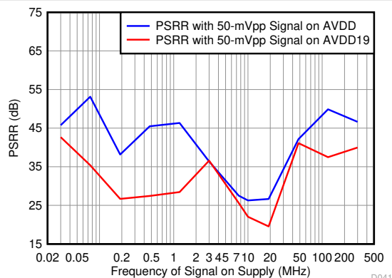
Figure 6-65. Power-Supply Rejection Ratio vs. Tone Frequency
