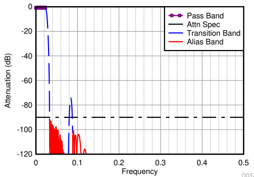
Figure 8-33. Divide-by-18 Filter Response
