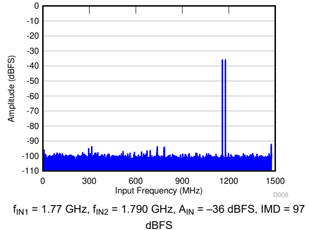
Figure 6-20. FFT for Two-Tone Input Signal (–36 dBFS)
