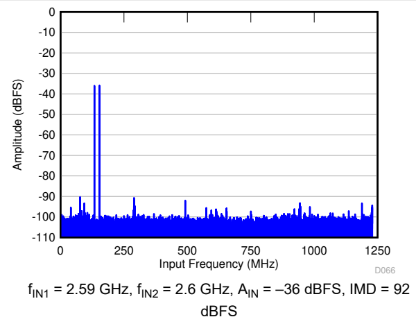
Figure 6-30. FFT for Two-Tone Input Signal (-36 dBFS, f_s = 2457.6 \text{ MSPS} )
