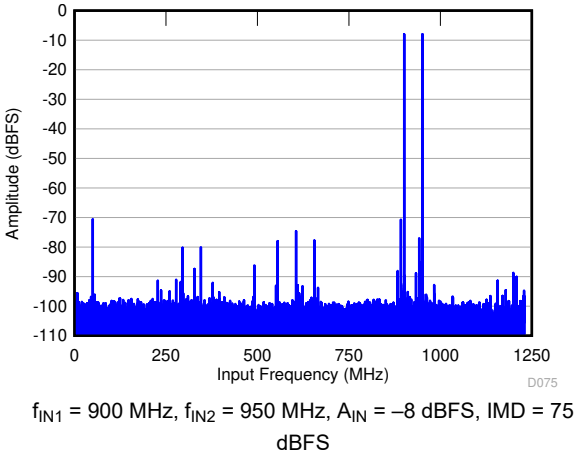
Figure 6-17. FFT for Two-Tone Input Signal (–8 dBFS, f_s = 2457.6 \text{ MSPS} )
