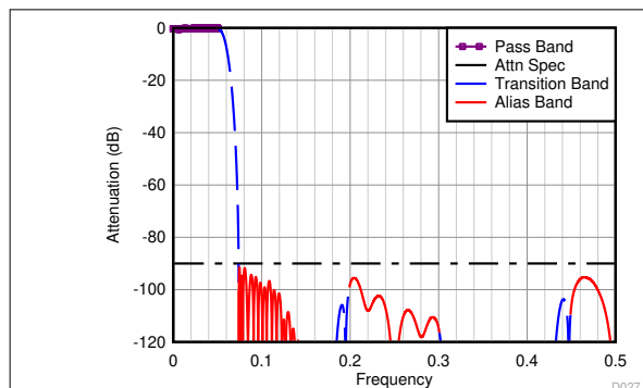
Figure 8-23. Divide-by-8 Filter Response
