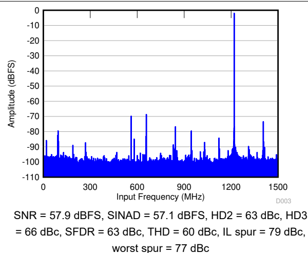
Figure 9-12. FFT for 1780-MHz Input Frequency
