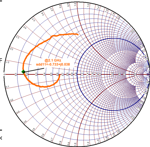
Figure 8-2. SDD11 Over the Input Frequency Range
