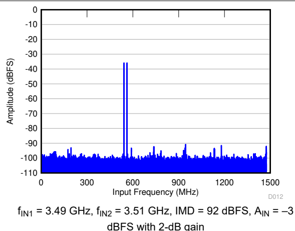
Figure 6-28. FFT for Two-Tone Input Signal (–36 dBFS)
