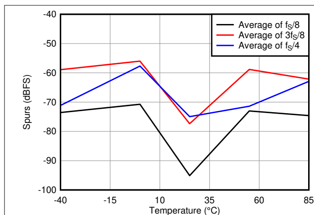
Figure 9-7. Offset Corrector Block Frozen at Room Temperature
