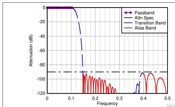
Figure 8-19. Divide-by-4 Filter Response
