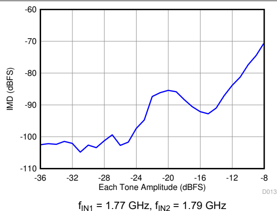
Figure 6-31. Intermodulation Distortion vs. Input Amplitude (1770 MHz and 1790 MHz)
