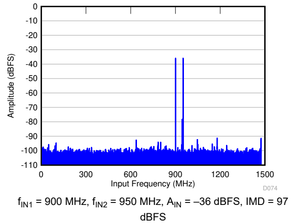
Figure 6-16. FFT for Two-Tone Input Signal (–36 dBFS)
