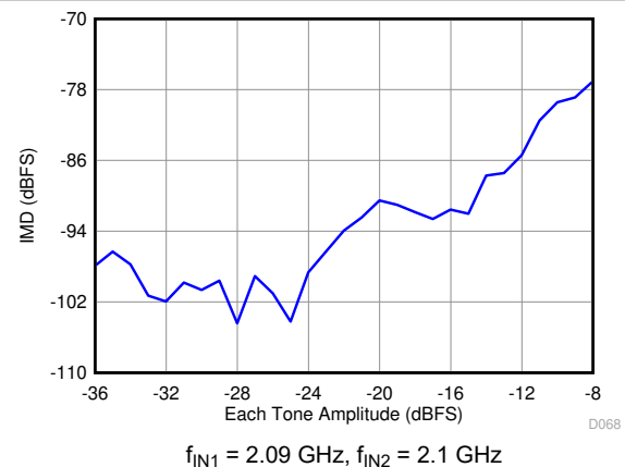
Figure 6-34. Intermodulation Distortion vs. Input Amplitude (1800 MHz and 2600 MHz, f_s = 2457.6 \text{ MSPS} )
