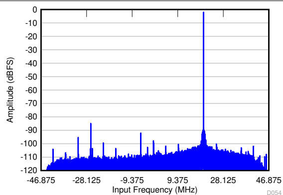
Figure 6-78. FFT in 32x Decimation (Complex Output)
