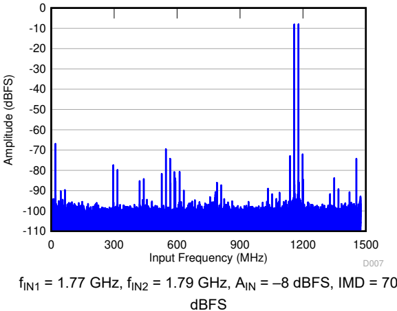
Figure 6-19. FFT for Two-Tone Input Signal (–8 dBFS)
