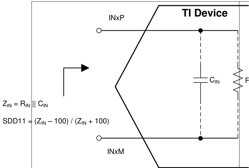
Copyright © 2016, Texas Instruments Incorporated Figure 8-1. Equivalent Input Impedance
