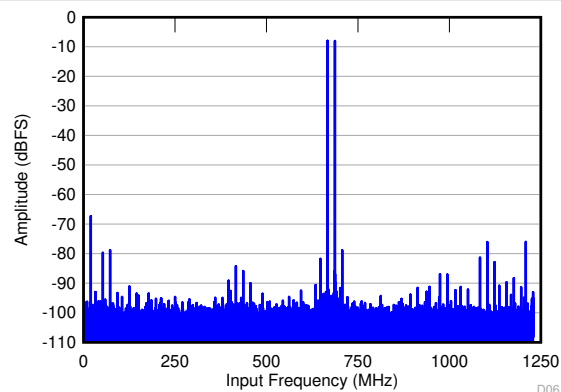
Figure 6-21. FFT for Two-Tone Input Signal (–8 dBFS, f_s = 2457.6 \text{ MSPS} )
