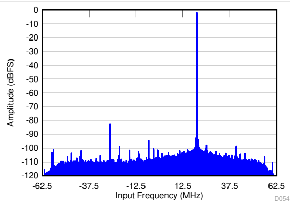
Figure 6-77. FFT in 24x Decimation (Complex Output)
