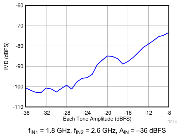
Figure 6-33. Intermodulation Distortion vs. Input Amplitude (1800 MHz and 2600 MHz)
