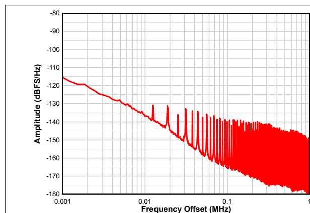
Figure 7-6. Dither Close-Up
