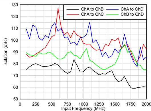
Figure 6-38. Isolation vs Input Frequency
