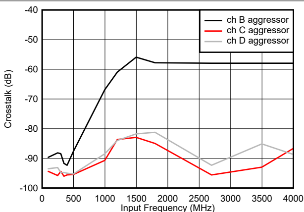
Figure 5-4. Crosstalk vs Input Frequency, Channel A victim
