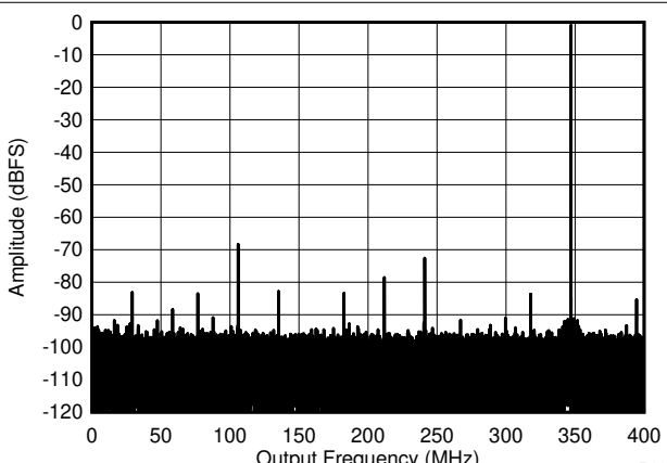
Figure 5-6. Single Tone FFT at 347 MHz and -1dBFS
