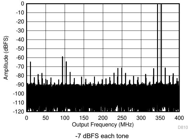
Figure 5-69. Two Tone FFT at 347 MHz in Low Power Mode
