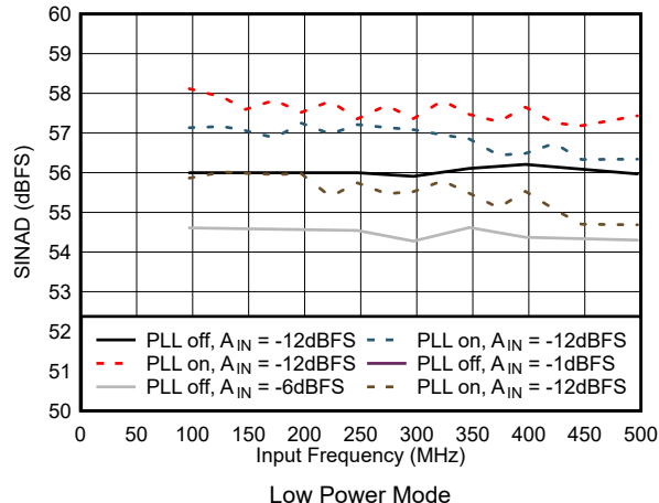
Figure 5-52. SINAD vs Input Frequency in Low Power Mode
