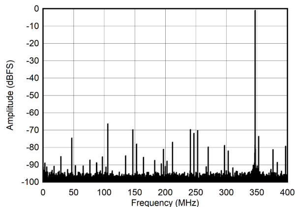
Figure 5-15. Single Tone FFT at 347 MHz and -1dBFS
