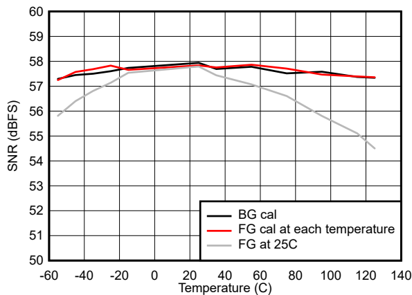
Figure 5-43. SNR vs Temperature F_{IN} = 347 MHz
