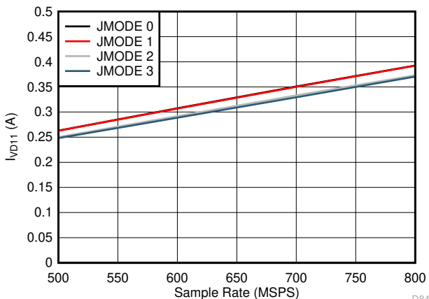
Independent of Power Mode Figure 5-80. Quad Channel, I_{VD11} vs F_S for JMODES 0 - 3
