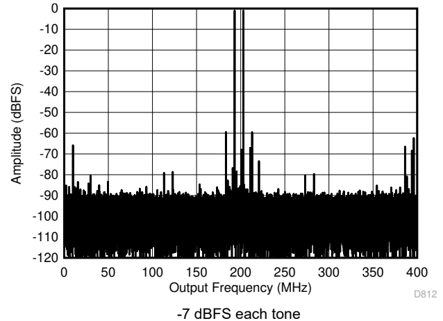
Figure 5-70. Two Tone FFT at 1798 MHz in Low Power Mode
