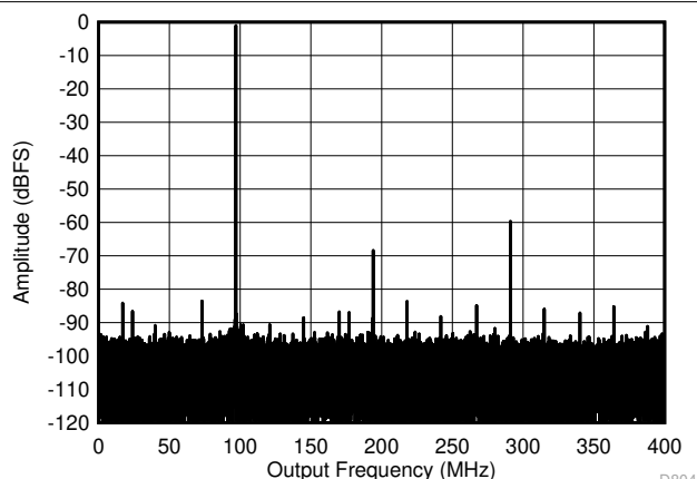
Figure 5-11. Single Tone FFT at 897 MHz and -1dBFS
