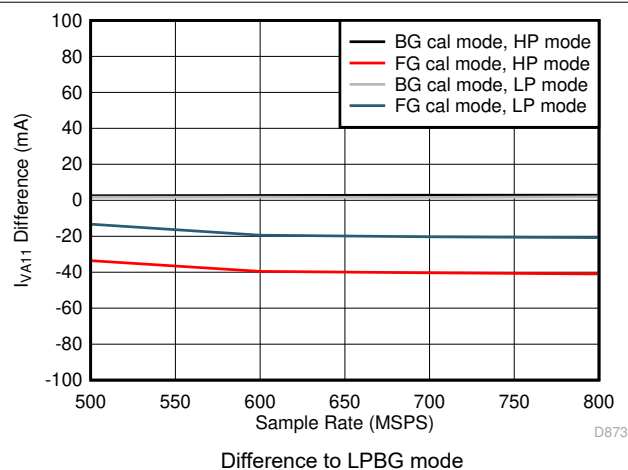
Figure 5-113. Single Channel, I_{VA11} vs F_S over Modes
