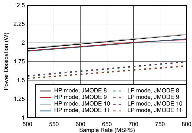
Figure 5-76. Quad Channel, Power Dissipation vs F_S for JMODES 8 - 11
