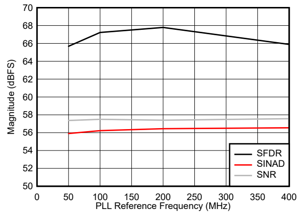
Figure 5-42. SNR, SFDR and SINAD vs Reference Frequency with PLL on
