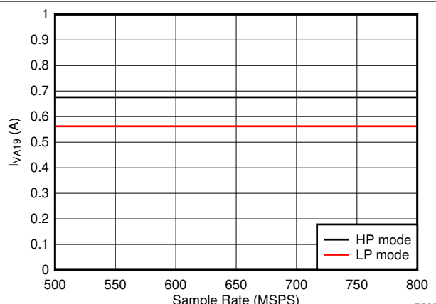
Independent of JMODE Figure 5-78. Quad Channel, I_{VA19} vs F_S
