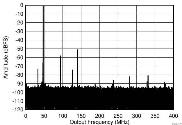
Figure 5-9. Single Tone FFT at 3247 MHz and -1dBFS
