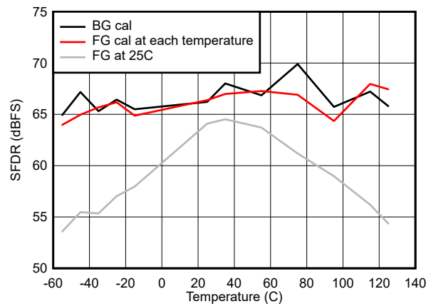
Figure 5-44. SFDR vs Temperature F_{IN} = 347 MHz
