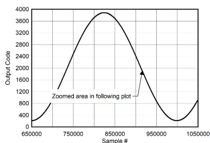
Figure 5-115. Background Calibration Core Transition (midscale)
