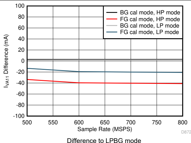
Figure 5-100. Dual Channel, I_{VA11} vs F_S over Modes
