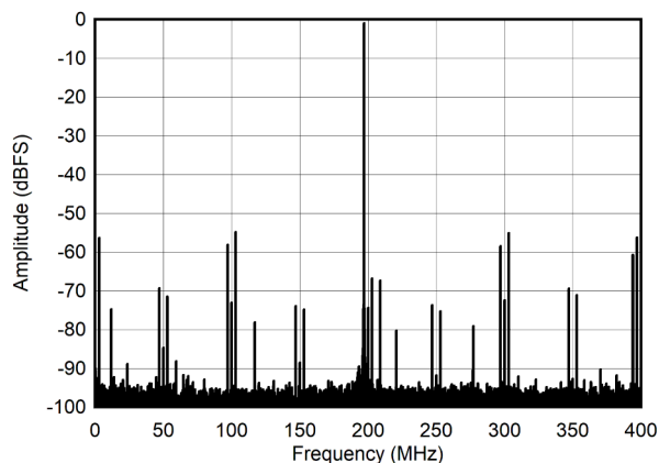
Figure 5-16. Single Tone FFT at 997 MHz and -1dBFS
