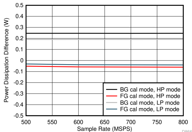
Figure 5-98. Dual Channel, Power Dissipation vs F_S over Modes
