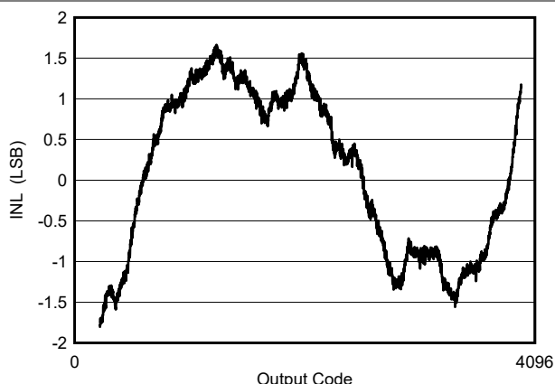
Figure 5-2. INL vs Code
