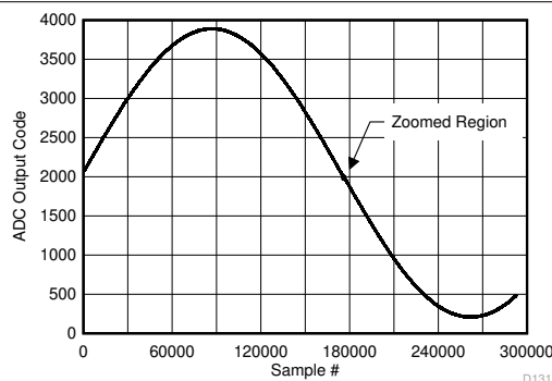
Figure 5-126. Background Calibration Core Transition (AC Signal)
