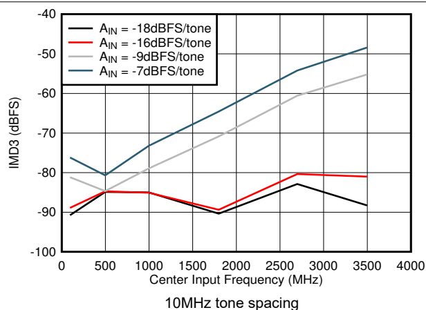
10MHz tone spacing Figure 5-75. IMD3 vs F_{IN}
