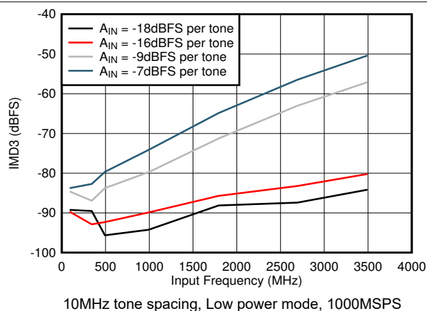
10MHz tone spacing, Low power mode, 1000MSPS Figure 5-76. IMD3 vs F_{IN}
