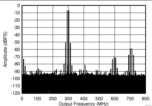
10MHz tone spacing Figure 5-71. Two Tone FFT at 3498MHz
