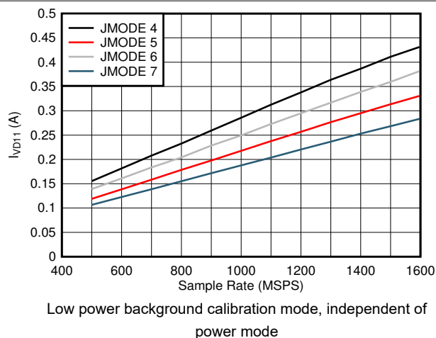
Figure 5-96. Dual Channel, Power Dissipation vs F_S and JMODE 4 - 7
