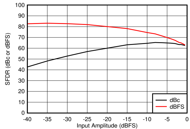
Figure 5-32. SFDR vs A_{IN}
