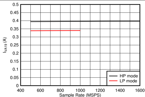
Figure 5-93. Dual Channel, I_{VA19} vs F_S
