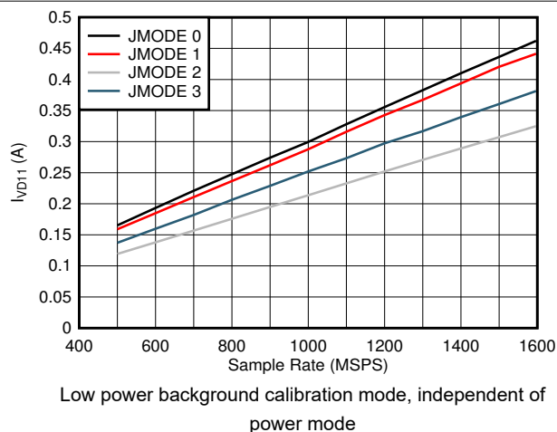
Figure 5-95. Dual Channel, Power Dissipation vs F_S and JMODE 0 - 3
