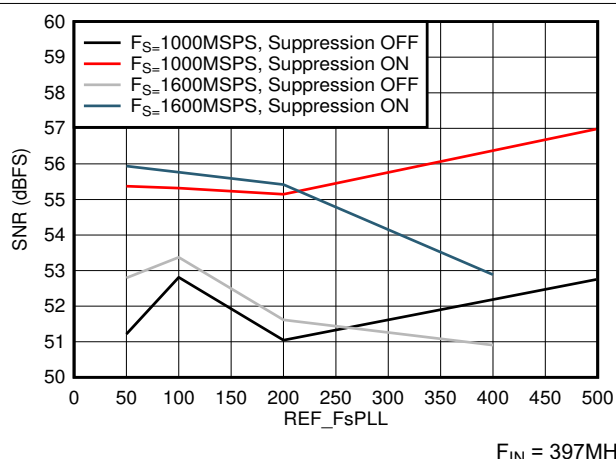
Figure 5-38. SNR vs F_{REF} and Suppression
