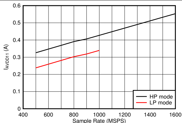
Figure 5-94. Dual Channel, I_{VA11} vs F_S
