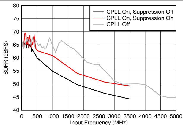
Figure 5-40. SFDR vs F_{IN} and C-PLL modes
