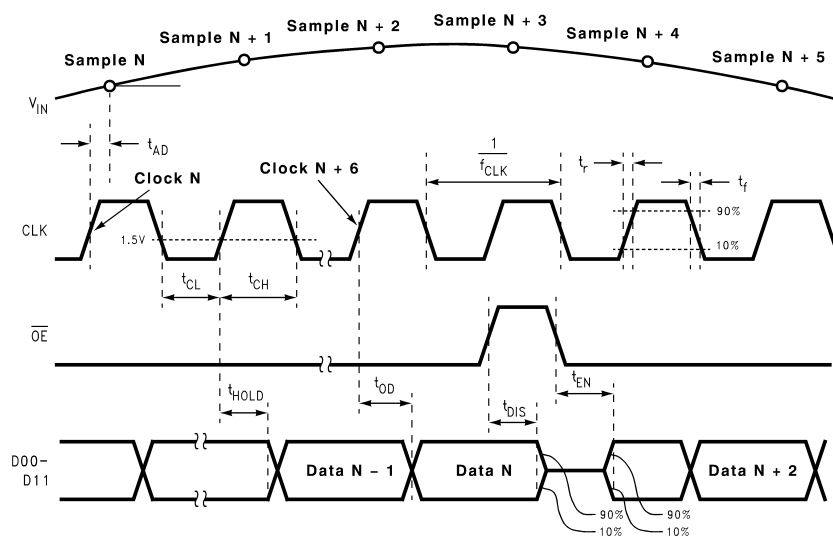
Figure 3. Output Timing
