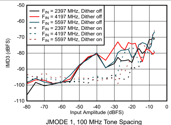
Figure 5-24. DES Mode: IMD3 vs Input Amplitude
