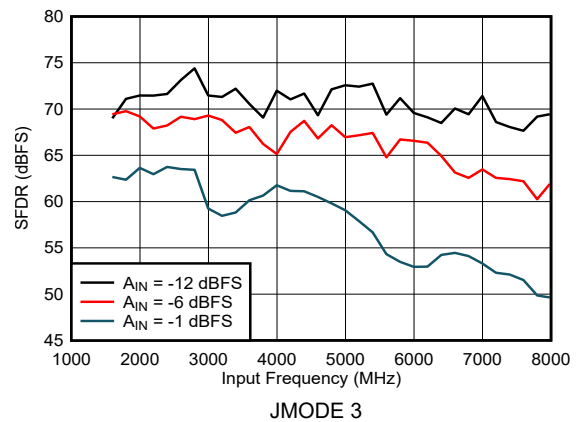
Figure 5-34. Dual Channel Mode: SFDR vs Input Frequency
