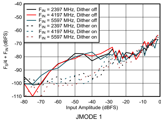
Figure 5-21. DES Mode: \text{FS}/4 + F_{\text{IN}} vs Input Amplitude
