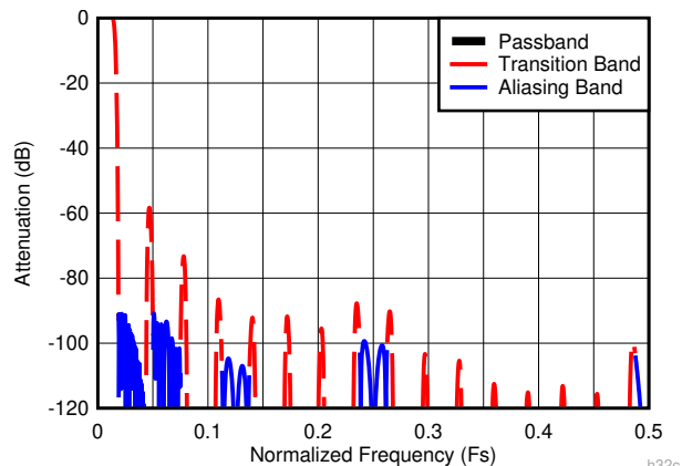
Figure 6-17. Decimate-by-32 Composite Response
