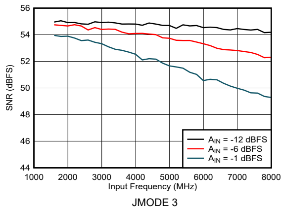
Figure 5-33. Dual Channel Mode: SNR vs Input Frequency
