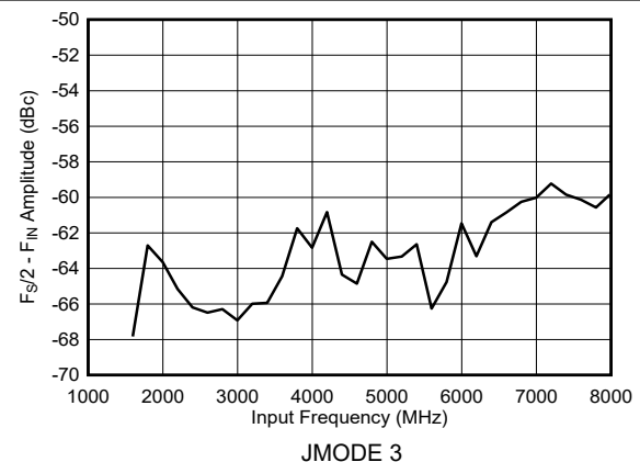
Figure 5-38. Dual Channel Mode: F_S/2 - F_{\text{IN}} vs Input Frequency
