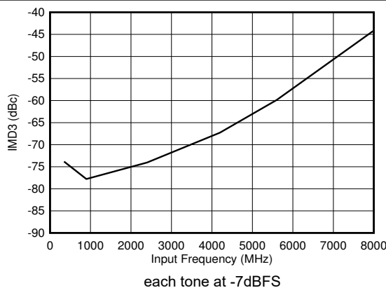
Figure 5-99. DES Mode: IMD3 vs Input Frequency
