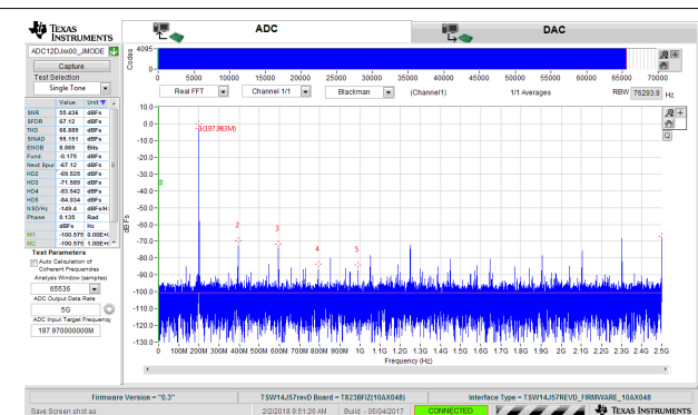
Figure 7-9. 200-MHz, Sine-Wave Frequency Domain (FFT) for 5-GSPS, Single-Channel Oscilloscope
