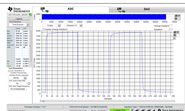
Figure 7-7. 40-MHz, Square-Wave Time Domain for 5-GSPS, Single-Channel Oscilloscope
