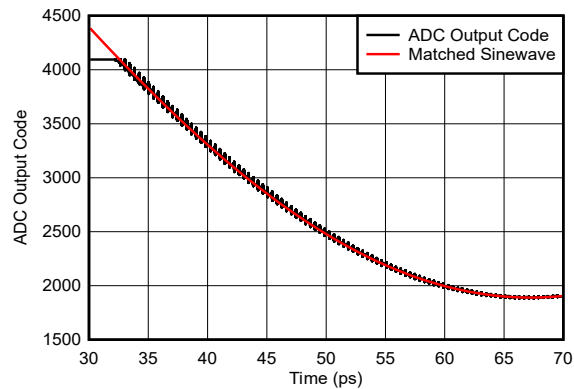
Figure 5-149. Sinewave Overdrive Recovery
