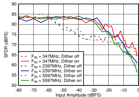
Figure 5-60. DES Mode: SFDR vs Input Amplitude and Dither
