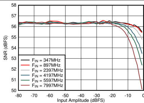
Figure 5-57. DES Mode: SNR vs Input Amplitude and Frequency
