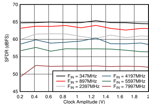
Figure 5-82. DES Mode: SFDR vs Clock Amplitude
