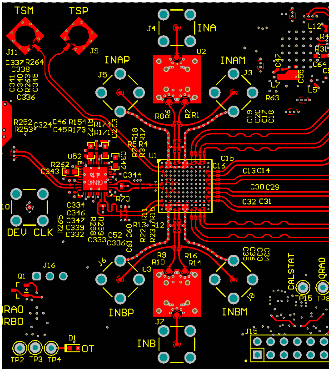
Figure 7-15. Top Layer Routing: Analog Inputs, CLK and SYSREF, DA0-3, DB0-3
