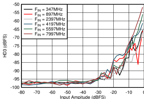
Figure 5-77. Dual Channel Mode: HD3 vs Input Amplitude and Frequency
