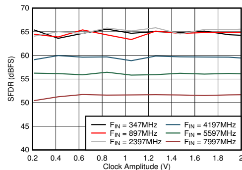
Figure 5-84. Dual Channel Mode: SFDR vs Clock Amplitude
