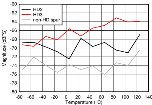
Figure 5-87. DES Mode: HD2, HD3 and Worst non-HD Spur vs Temperature
