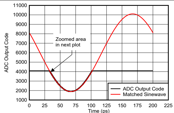
Figure 5-148. Sinewave Overdrive Recovery
