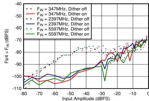
Figure 5-68. DES Mode: \text{Fs}/4 + F_{\text{IN}} vs Input Amplitude and Dither
