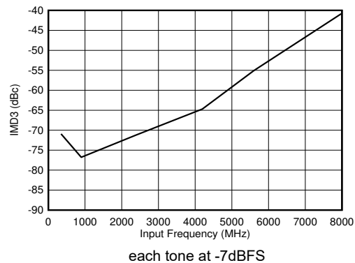
Figure 5-104. Dual Channel Mode: IMD3 vs Input Frequency
