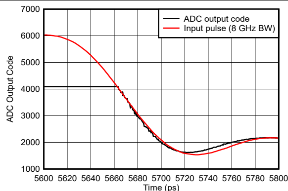
Figure 5-147. Pulse Overdrive Recovery Zoomed
