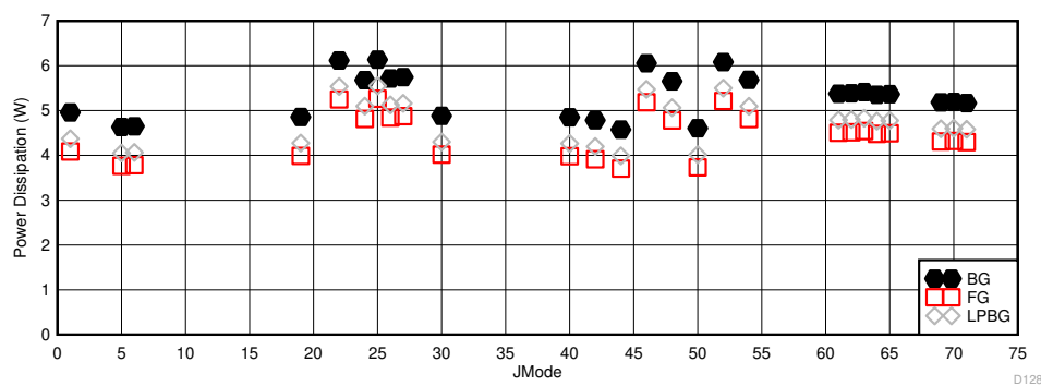
Figure 5-111. DES Mode: I_{VD11} vs JMODE at 10.4GSPS
