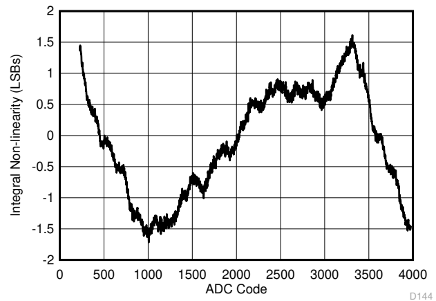
Figure 5-4. INL vs ADC Code
