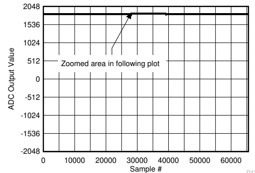
Figure 5-144. Background Calibration Core Transition (DC Signal)
