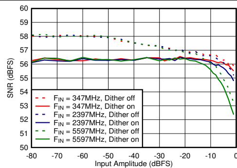
Figure 5-58. DES Mode: SNR vs Input Amplitude and Dither
