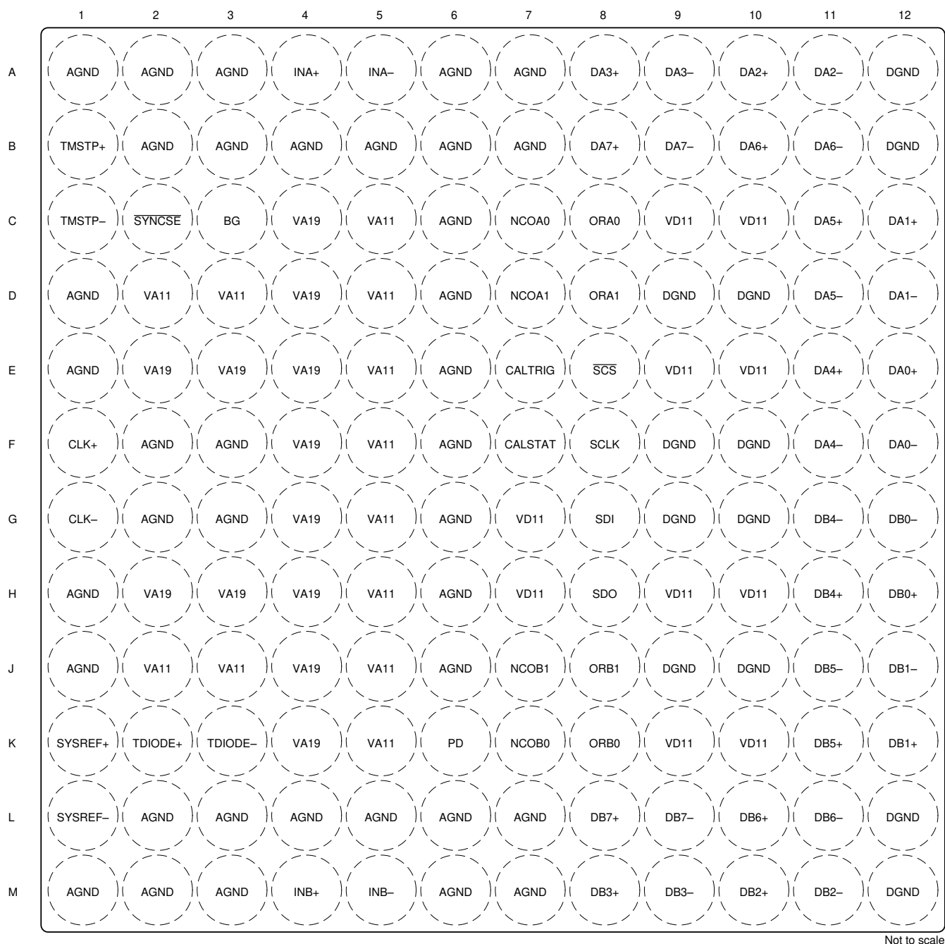
Figure 4-1. AAV Package, 144-Ball Flip Chip BGA Top View
