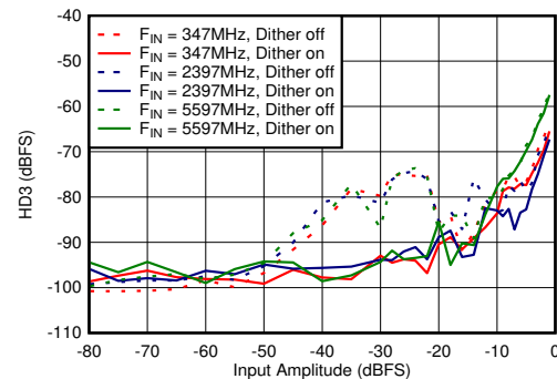
Figure 5-64. DES Mode: HD3 vs Input Amplitude and Dither
