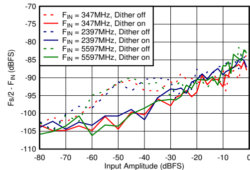
Figure 5-80. Dual Channel Mode: F_s/2 - F_{\text{IN}} vs Input Amplitude and Dither
