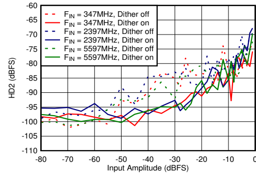
Figure 5-62. DES Mode: HD2 vs Input Amplitude and Dither
