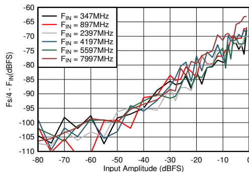
Figure 5-69. DES Mode: \text{Fs}/4 - F_{\text{IN}} vs Input Amplitude and Frequency
