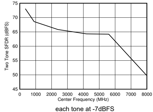
Figure 5-102. DES Mode: Two Tone SFDR vs Input Frequency
