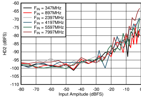
Figure 5-61. DES Mode: HD2 vs Input Amplitude and Frequency
