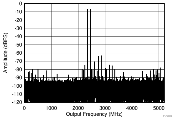
Figure 5-13. DES Mode: Two Tone FFT at 2397 MHz
