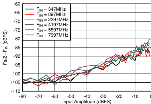
Figure 5-79. Dual Channel Mode: F_s/2 - F_{\text{IN}} vs Input Amplitude and Frequency
