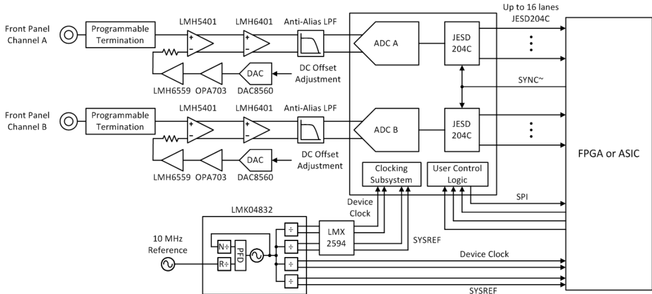
Figure 7-5. Typical Configuration for Reconfigurable Oscilloscope
