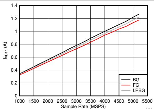
Figure 5-133. Dual Channel Mode: I_{VD11} vs Sample Rate
