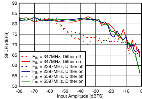
Figure 5-74. Dual Channel Mode: SFDR vs Input Amplitude and Dither
