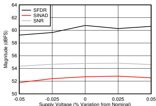
Figure 5-93. DES Mode: SNR, SINAD and SFDR vs Supply Voltage
