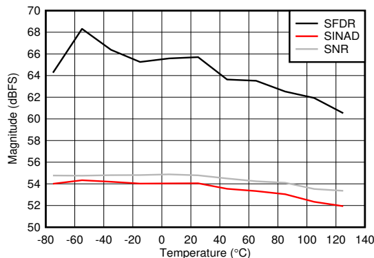
Figure 5-89. Dual Channel Mode: SNR, SINAD and SFDR vs Temperature
