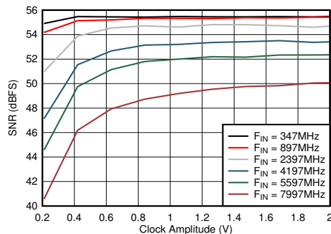
Figure 5-81. DES Mode: SNR vs Clock Amplitude
