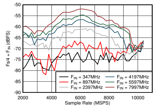
Figure 5-42. DES Mode: F_s/4 + F_{\text{IN}} vs Sample Rate and Input Frequency
