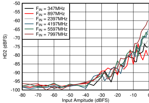
Figure 5-75. Dual Channel Mode: HD2 vs Input Amplitude and Frequency
