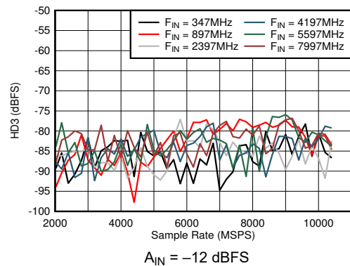
Figure 5-40. DES Mode: HD3 vs Sample Rate and Input Frequency
