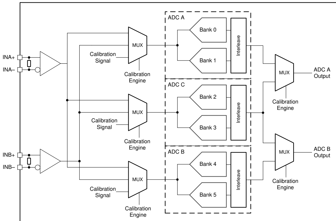
Figure 6-26. ADC12DJ5200RF Calibration System Block Diagram
