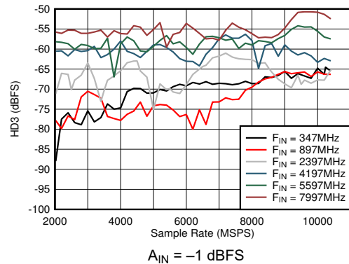
Figure 5-38. DES Mode: HD3 vs Sample Rate and Input Frequency
