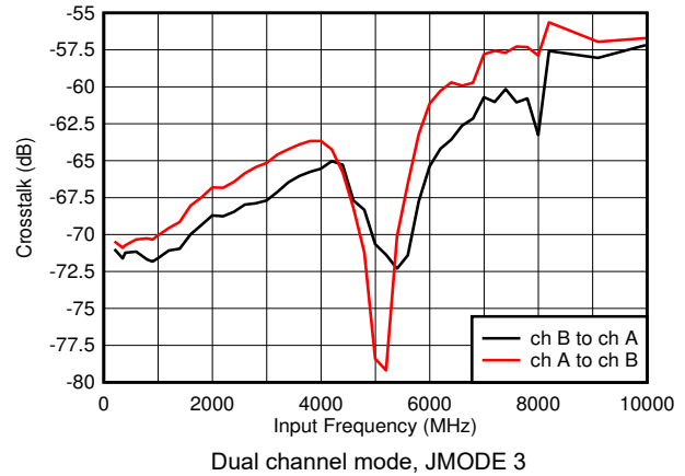
Figure 5-2. Crosstalk vs Input Frequency
