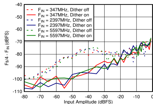
Figure 5-70. DES Mode: \text{Fs}/4 - F_{\text{IN}} vs Input Amplitude and Dither
