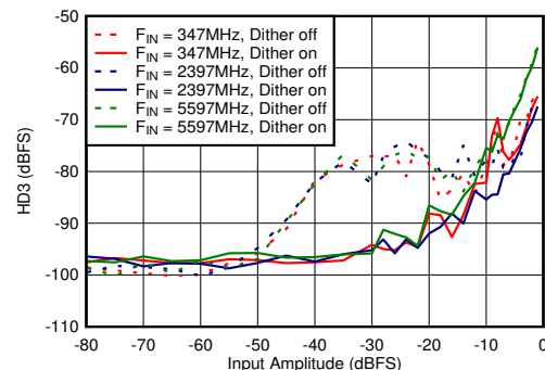
Figure 5-78. Dual Channel Mode: HD3 vs Input Amplitude and Dither
