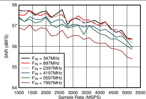
Figure 5-44. Dual Channel Mode: SNR vs Sample Rate and Input Frequency
