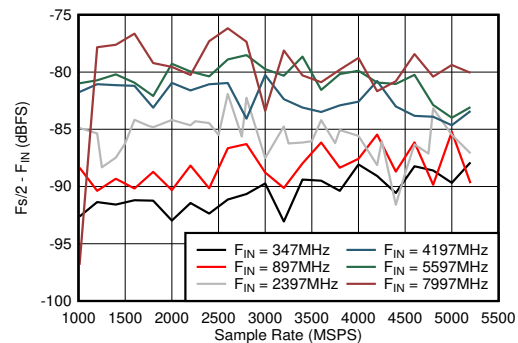
Figure 5-56. Dual Channel Mode: F_s/2 - F_{\text{IN}} vs Sample Rate and Input Frequency
