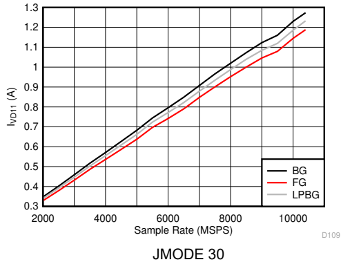
Figure 5-125. DES Mode: I_{VD11} vs Sample Rate
