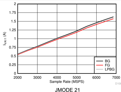
Figure 5-124. DES Mode: I_{VD11} vs Sample Rate
