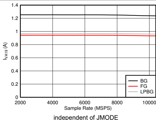
Figure 5-121. DES Mode: I_{VA19} vs Sample Rate
