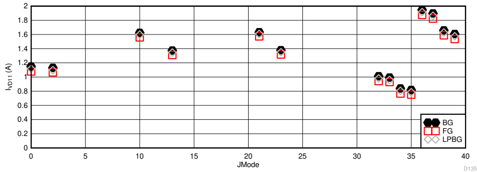
Figure 5-118. Other Modes with Lower Maximum F_S : I_{VA11} vs JMODE
