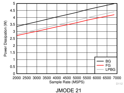
Figure 5-128. DES Mode: Power Dissipation vs Sample Rate
