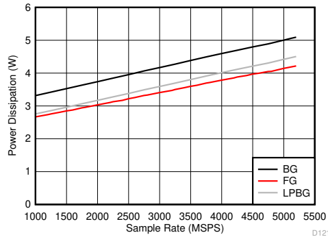
Figure 5-137. Dual Channel Mode: Power Dissipation vs Sample Rate
