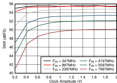
Figure 5-83. Dual Channel Mode: SNR vs Clock Amplitude
