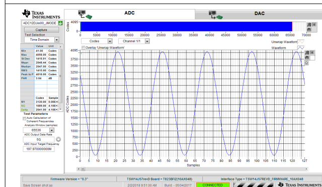
Figure 7-8. 200-MHz, Sine-Wave Time Domain for 5-GSPS, Single-Channel Oscilloscope
