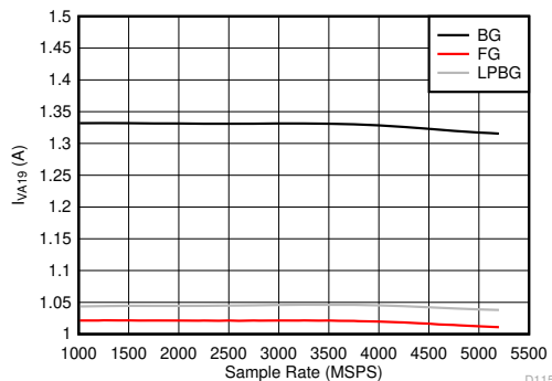
Figure 5-131. Dual Channel Mode: I_{VA19} vs Sample Rate
