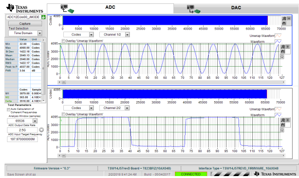
Figure 7-11. 200-MHz, Sine-Wave (Channel A) and 40-MHz, Square-Wave (Channel B) Time Domain for 5-GSPS, Single-Channel Oscilloscope
