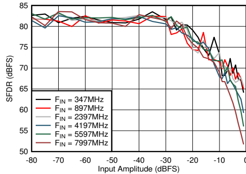
Figure 5-73. Dual Channel Mode: SFDR vs Input Amplitude and Frequency
