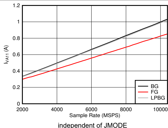
Figure 5-122. DES Mode: I_{VA11} vs Sample Rate
