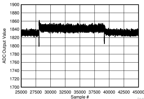
Figure 5-145. Background Calibration Core Transition (DC Signal - zoomed)
