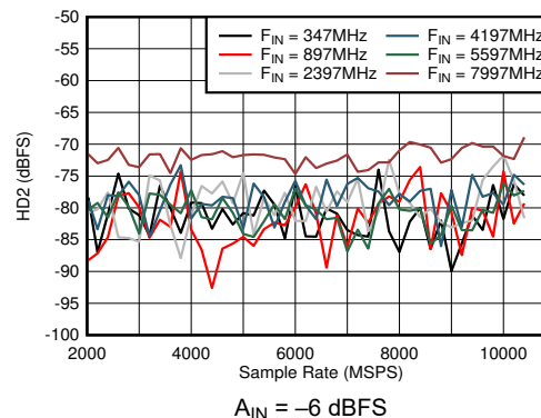
Figure 5-36. DES Mode: HD2 vs Sample Rate and Input Frequency
