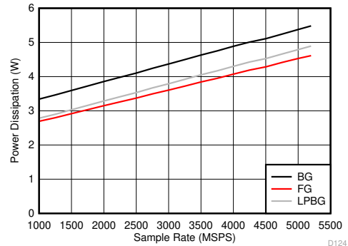
Figure 5-138. Dual Channel Mode: Power Dissipation vs Sample Rate
