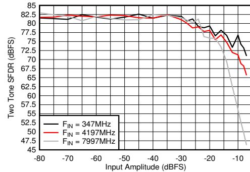
Figure 5-108. Dual Channel Mode: Two Tone SFDR vs Input Amplitude
