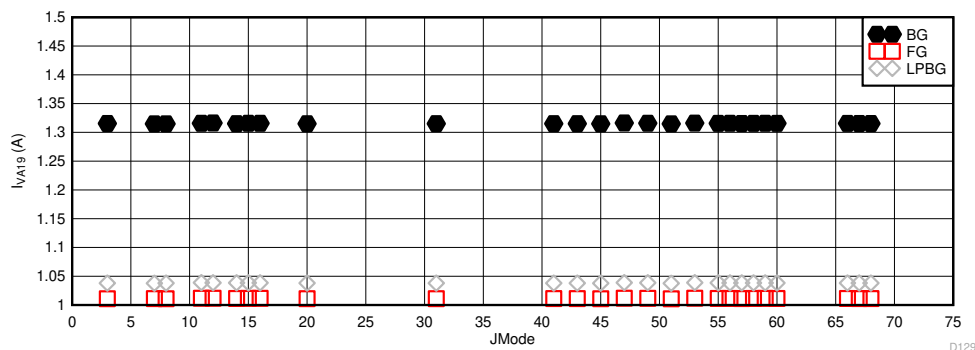
Figure 5-112. DES Mode: Power Dissipation vs JMODE at 10.4GSPS
