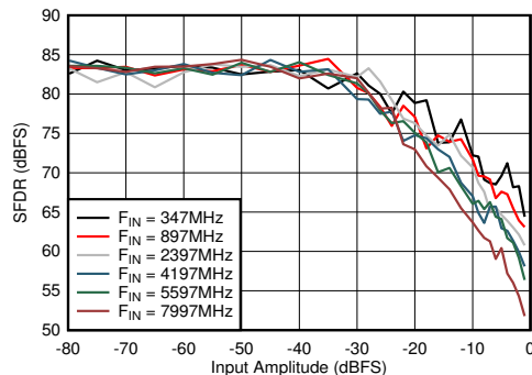
Figure 5-59. DES Mode: SFDR vs Input Amplitude and Frequency
