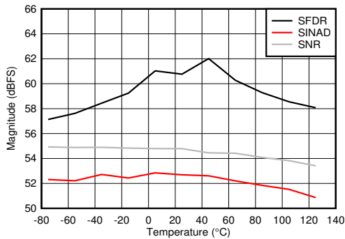
Figure 5-85. DES Mode: SNR, SINAD and SFDR vs Temperature
