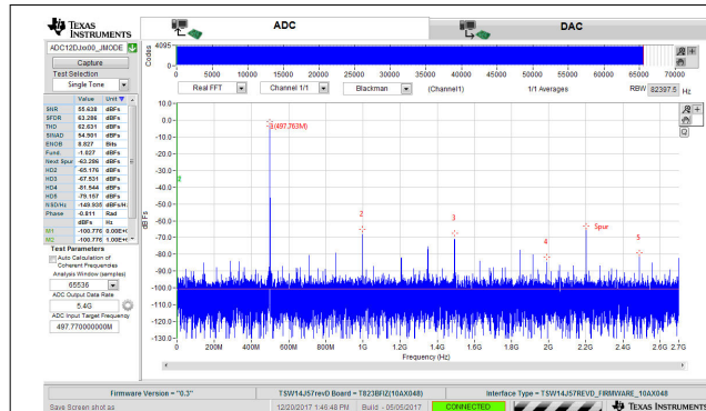
Figure 7-2. FFT for 497.77-MHz Input Signal, 5.4 GSPS, JMODE0
