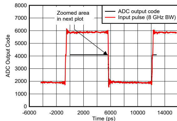
Figure 5-146. Pulse Overdrive Recovery
