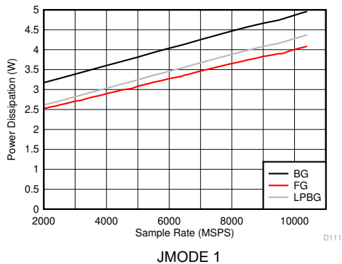
Figure 5-127. DES Mode: Power Dissipation vs Sample Rate
