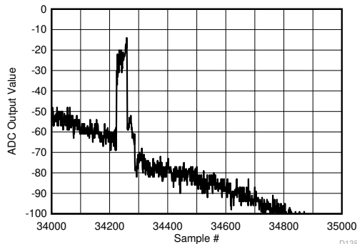
Figure 5-143. Background Calibration Core Transition (AC Signal - zoomed)
