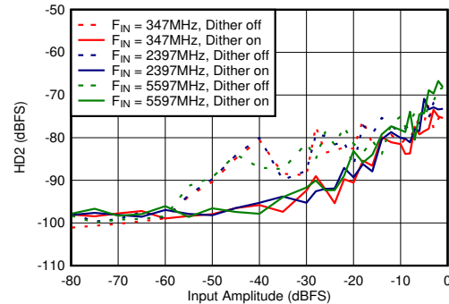
Figure 5-76. Dual Channel Mode: HD2 vs Input Amplitude and Dither
