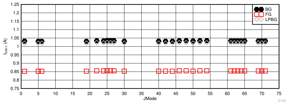
Figure 5-109. DES Mode: I_{VA19} vs JMODE at 10.4GSPS
