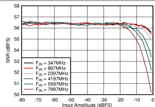
Figure 5-71. Dual Channel Mode: SNR vs Input Amplitude and Frequency
