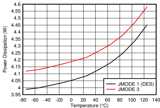
Figure 5-141. Power Dissipation vs Temperature
