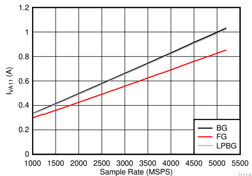
Figure 5-132. Dual Channel Mode: I_{VA11} vs Sample Rate
