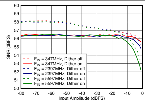
Figure 5-72. Dual Channel Mode: SNR vs Input Amplitude and Dither
