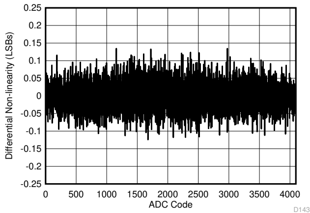
Figure 5-3. DNL vs ADC Code
