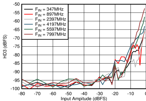
Figure 5-63. DES Mode: HD3 vs Input Amplitude and Frequency
