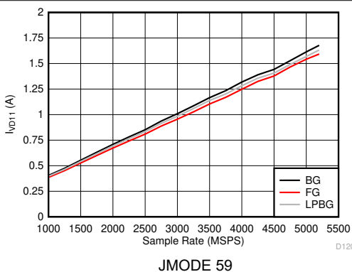
Figure 5-138. Dual Channel Mode: I_{VD11} vs Sample Rate
