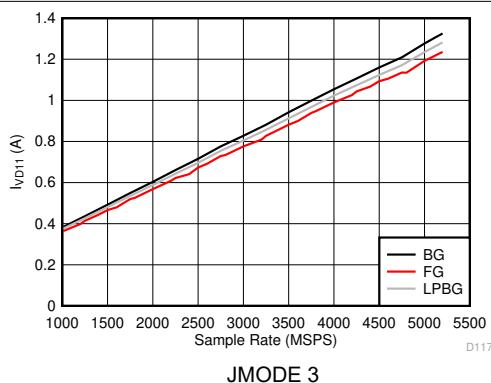
Figure 5-135. Dual Channel Mode: I_{VD11} vs Sample Rate
