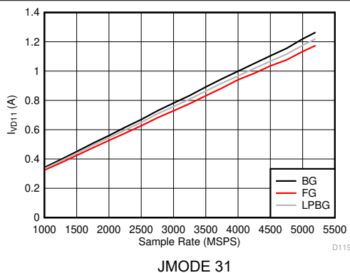
Figure 5-137. Dual Channel Mode: I_{VD11} vs Sample Rate
