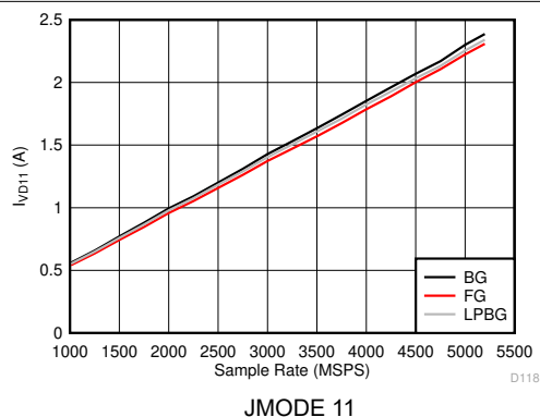
Figure 5-136. Dual Channel Mode: I_{VD11} vs Sample Rate
