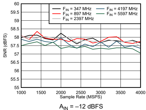
Figure 6-44. Dual Channel Mode: SNR vs Sample Rate and Input Frequency
