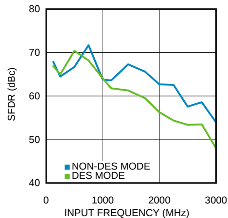
Figure 4-30. SFDR vs Input Frequency (ADC12D1000RF)
