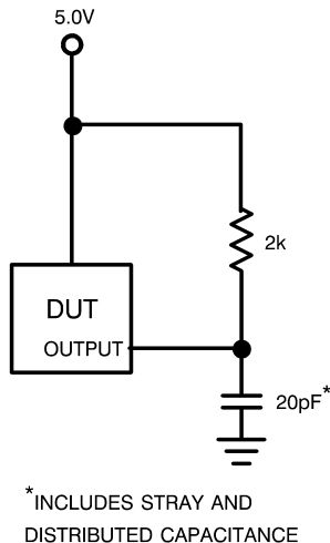
Figure 18. AC Test Circuit
