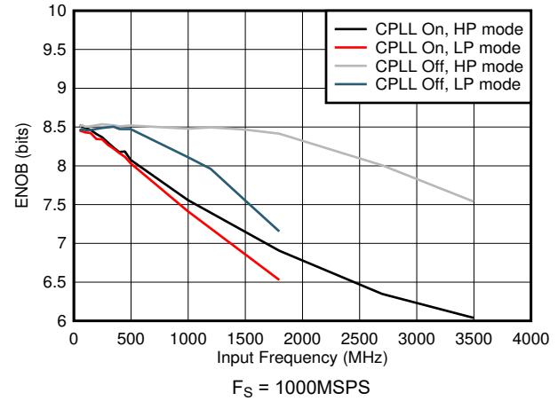
Figure 5-68. ENOB vs Input Frequency and CPLL
