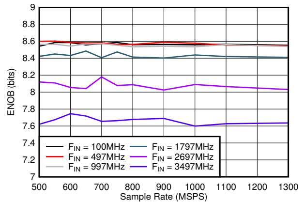
Figure 5-24. ENOB vs Sample Rate
