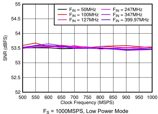
Figure 5-26. SNR vs Sample Rate
