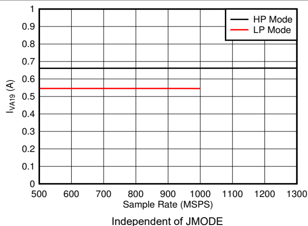
Figure 5-85. Quad Channel, I_{VA19} vs FS
