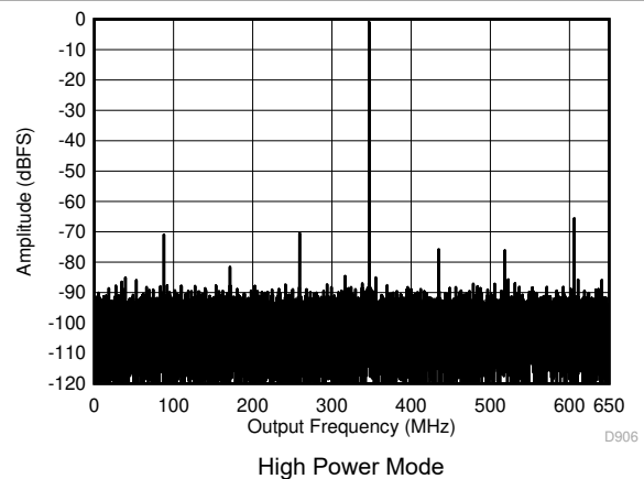
Figure 5-4. Single Tone FFT at 347 MHz and -1 dBFS
