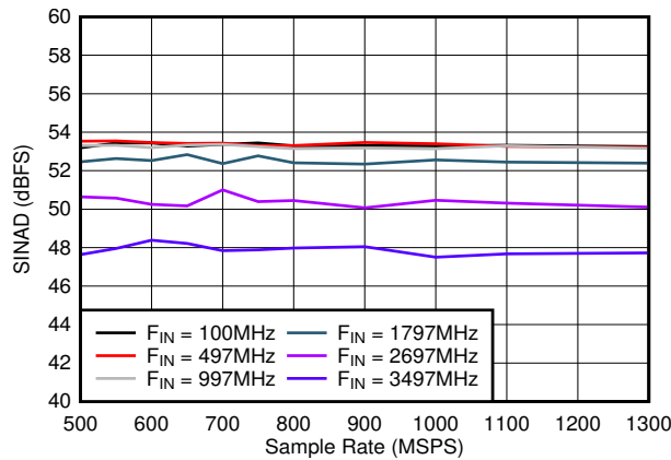
Figure 5-23. SINAD vs Sample Rate
