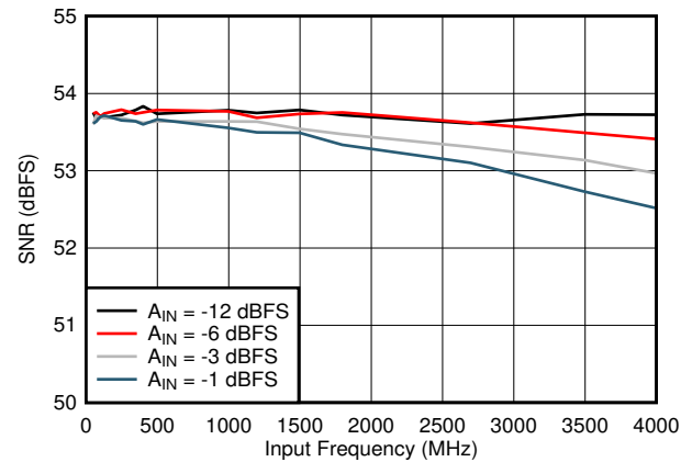
Figure 5-16. SNR vs Input Frequency
