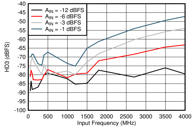
Figure 5-20. HD3 vs Input Frequency
