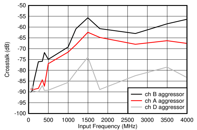
Figure 5-60. Crosstalk to Channel B vs F_{IN}
