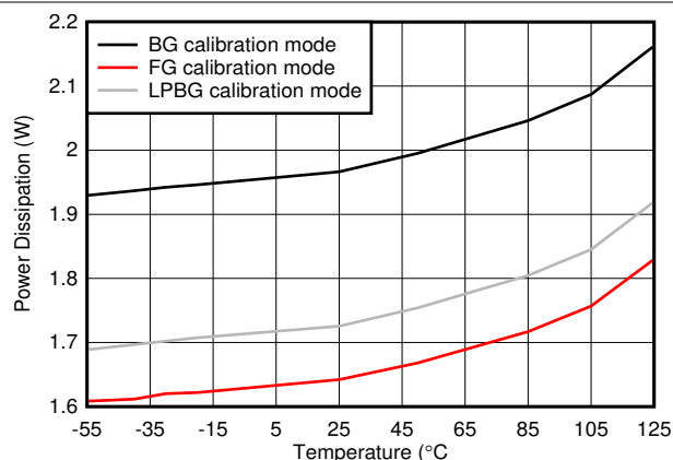
Figure 5-124. Dual Channel, Power Dissipation vs Temperature
