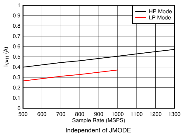
Figure 5-86. Quad Channel, I_{VA11} vs FS
