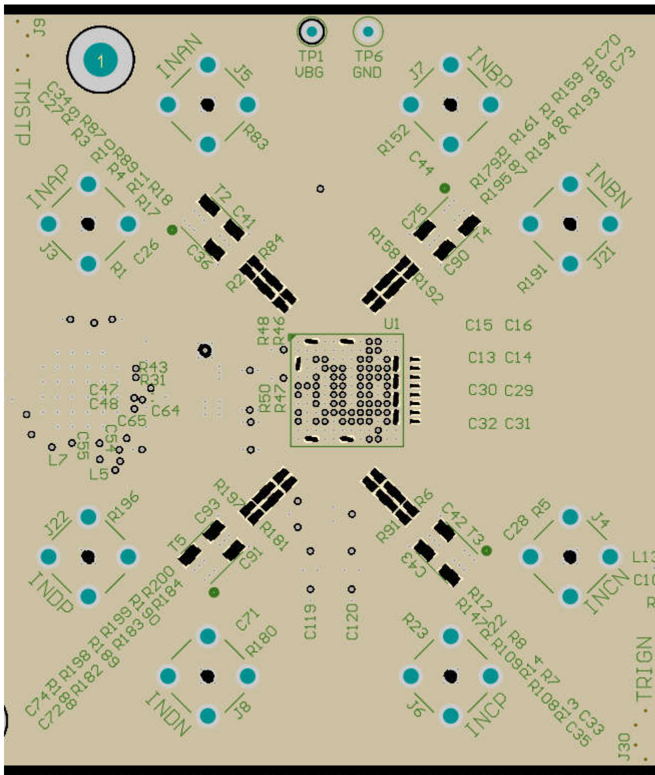
Figure 7-6. GND1 Cutouts to Optimize Impedance of Component Pads
