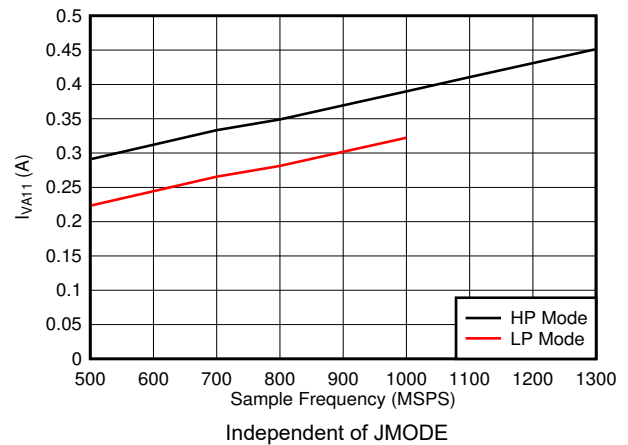
Figure 5-96. Dual Channel, I_{VA11} vs FS
