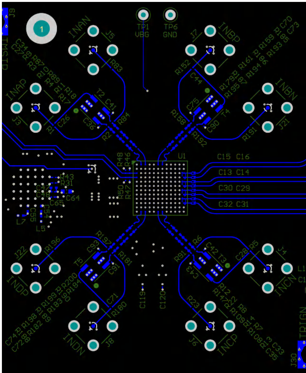
Figure 7-5. Top Layer Routing: Analog Inputs (INA±, INB±, INC±, IND±), TMSTP± and D[3:0]± Routing
