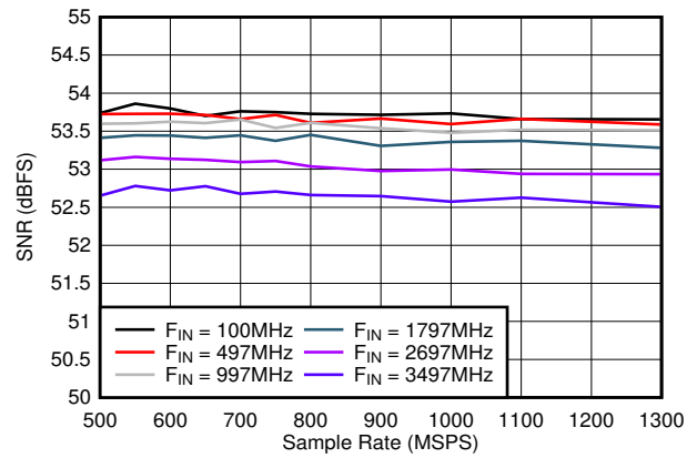
Figure 5-22. SNR vs Sample Rate
