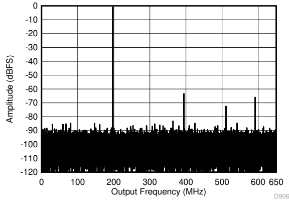
Figure 5-7. Single Tone FFT at 1497 MHz and -1 dBFS
