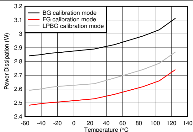
Figure 5-123. Quad Channel, Power Dissipation vs Temperature
