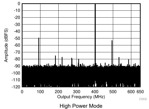
Figure 5-10. Single Tone FFT at 3497 MHz and -1 dBFS
