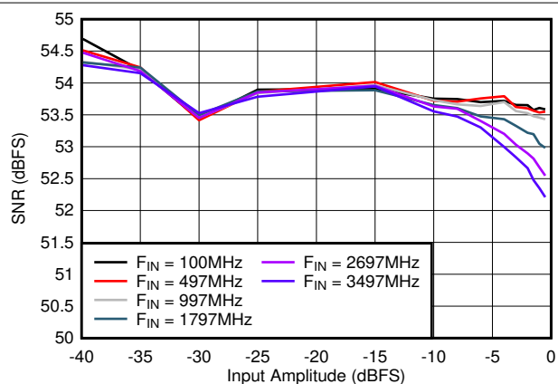
Figure 5-30. SNR vs Input Amplitude
