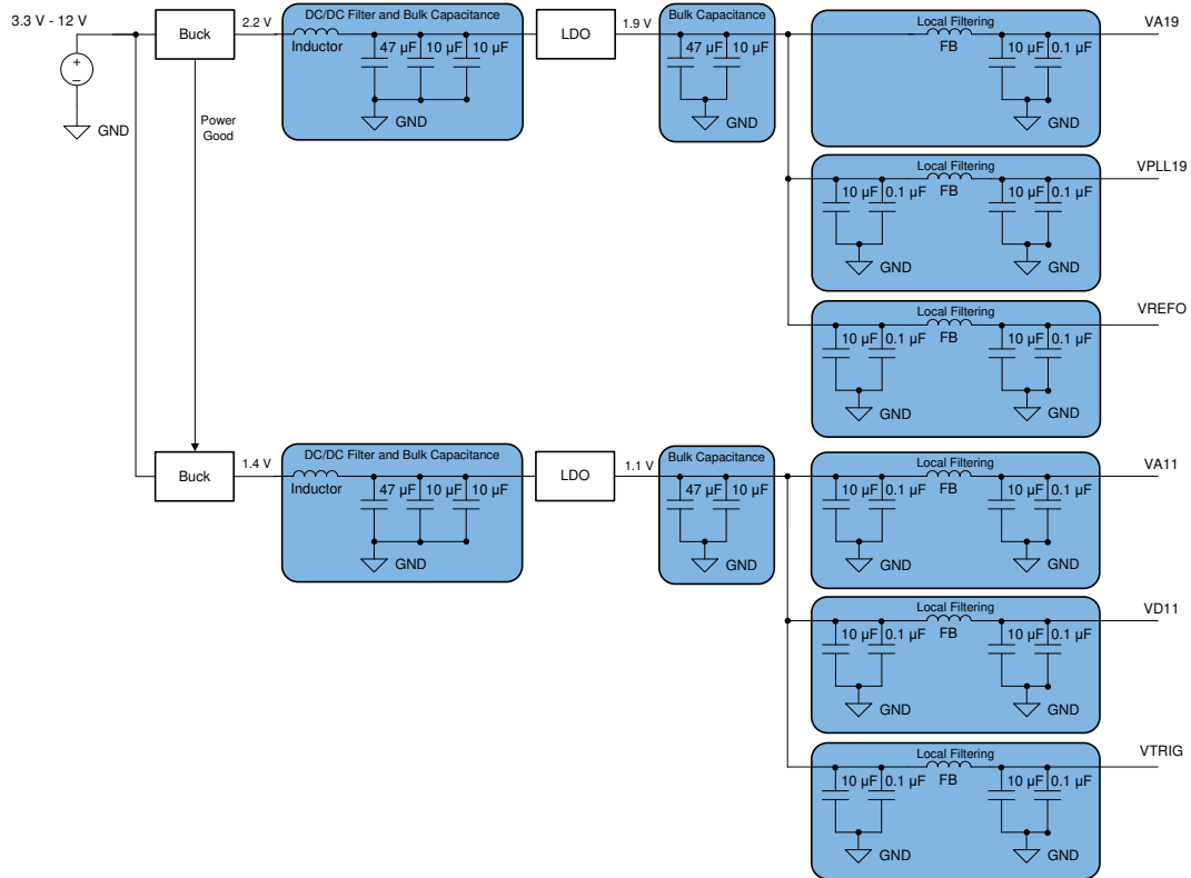
Figure 7-3. LDO Linear Regulator Approach Example
