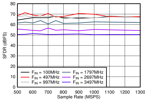
Figure 5-21. SFDR vs Sample Rate
