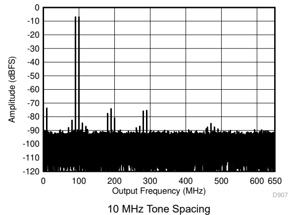
Figure 5-48. Two Tone FFT at 95.07 MHz Center
