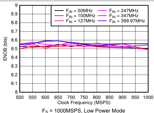
Figure 5-28. ENOB vs Sample Rate
