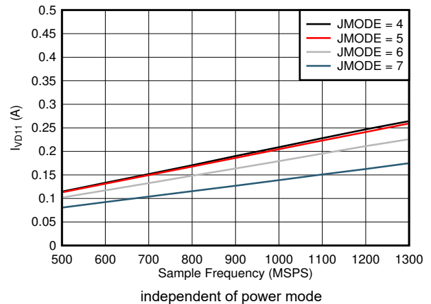
Figure 5-108. Single Channel, I_{VD11} vs FS and JMODE 4 - 7
