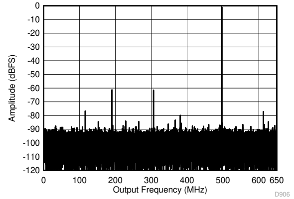
Figure 5-8. Single Tone FFT at 1797 MHz and -1 dBFS
