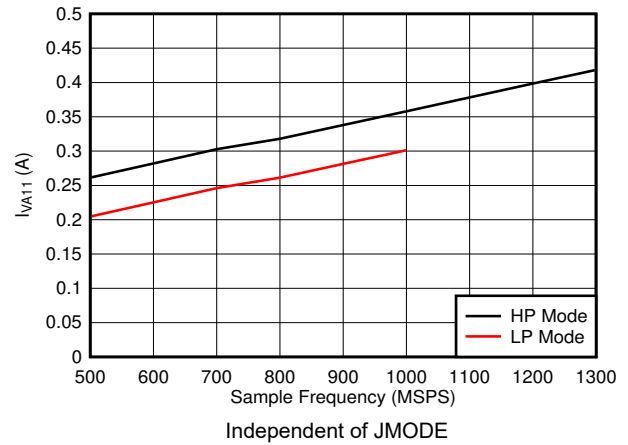
Figure 5-106. Single Channel, I_{VA11} vs FS
