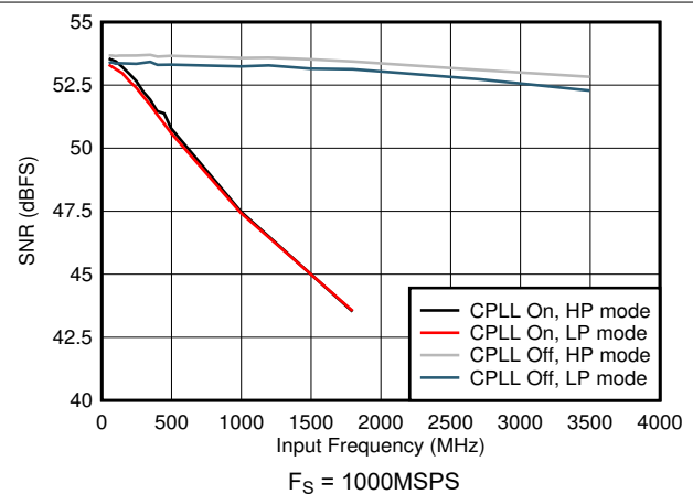
Figure 5-66. SNR vs Input Frequency and CPLL
