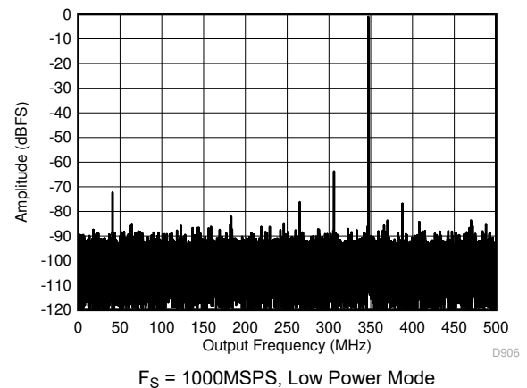
Figure 5-12. Single Tone FFT at 347 MHz and -1 dBFS
