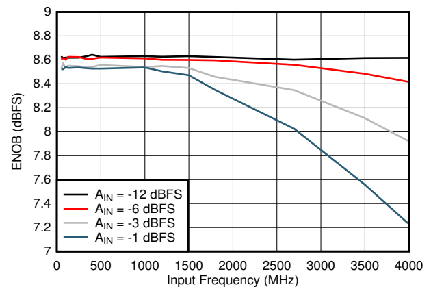
Figure 5-18. ENOB vs Input Frequency
