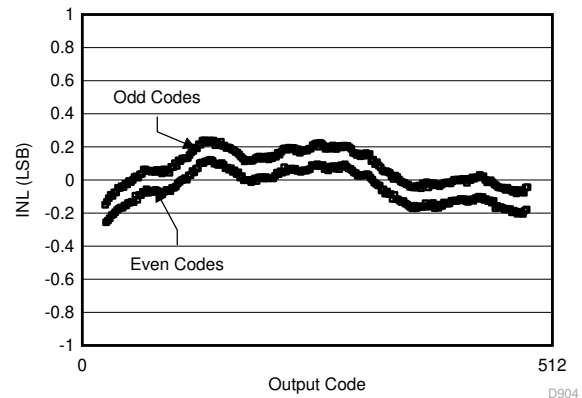
Figure 5-2. INL vs Code
