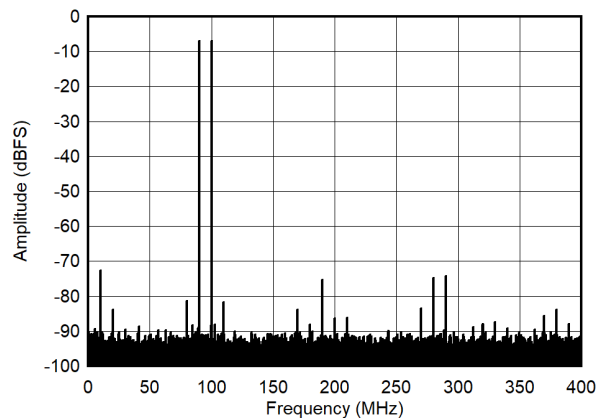
Figure 5-56. Dual Tone FFT at 95 MHz (LP Mode)
