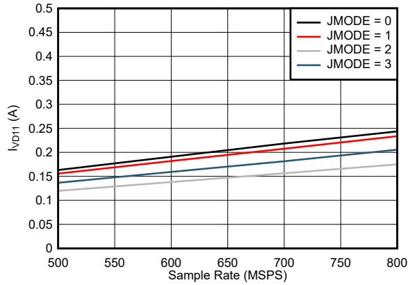
Figure 5-87. Dual Channel, I_{VD11} vs F_S for JMODES 0 - 3
