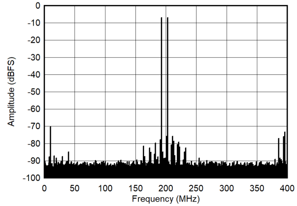
Figure 5-58. Dual Tone FFT at 998 MHz (LP Mode)
