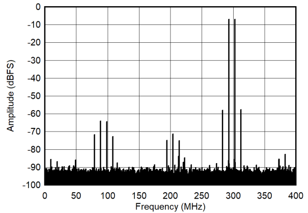
Figure 5-54. Dual Tone FFT at 2698 MHz
