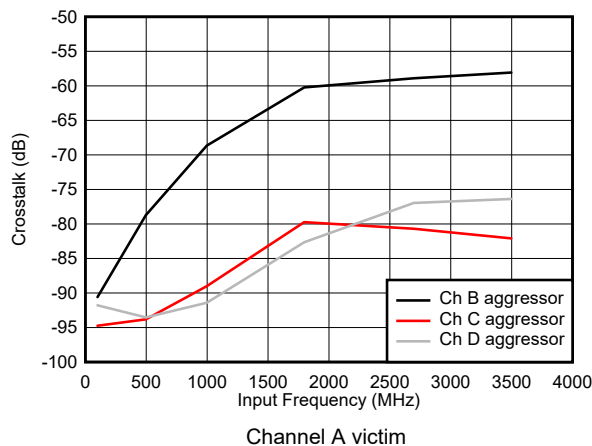
Figure 5-61. Crosstalk vs Input Frequency
