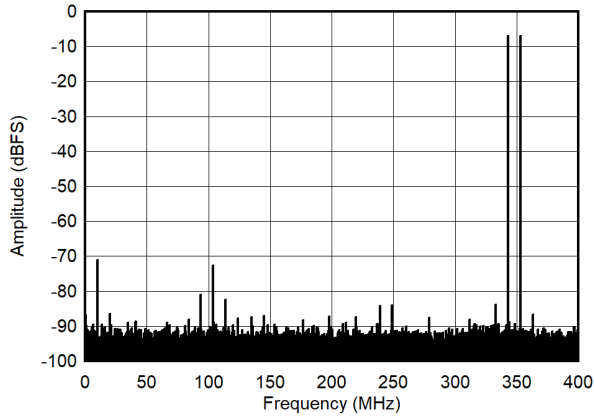
Figure 5-57. Dual Tone FFT at 348 MHz (LP Mode)
