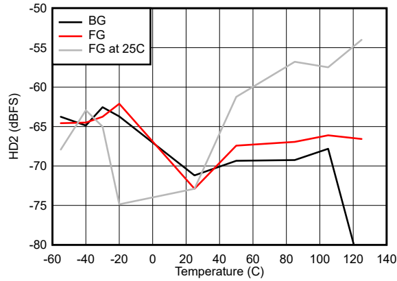
Figure 5-43. HD2 vs Temperature
