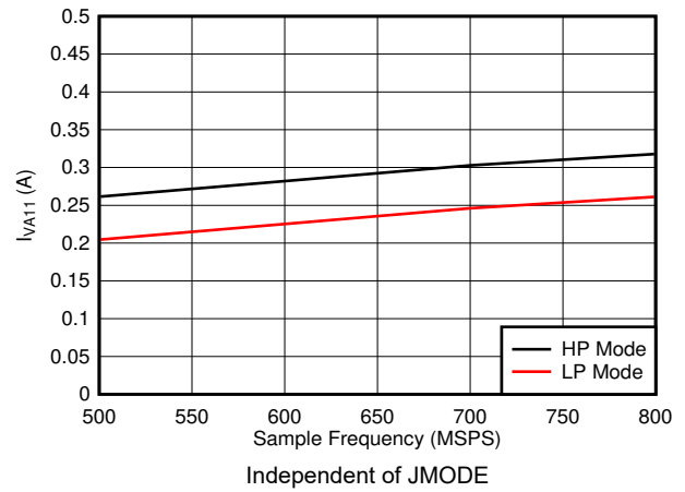
Figure 5-96. Single Channel, I_{VA11} vs F_S
