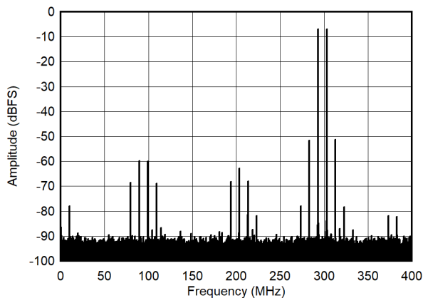
Figure 5-55. Dual Tone FFT at 2698 MHz
