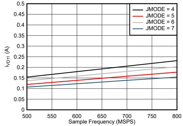
Figure 5-88. Dual Channel, I_{VD11} vs F_S for JMODES 4 - 7
