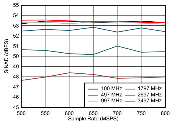
Figure 5-22. SINAD vs Sample Rate
