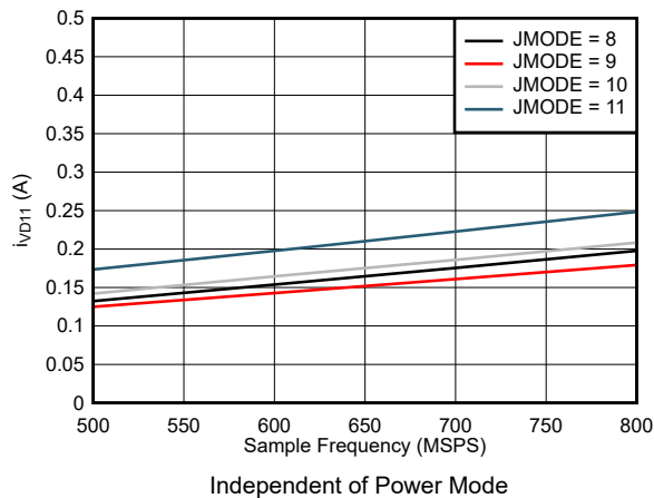
Figure 5-89. Dual Channel, I_{VD11} vs F_S for JMODES 8 - 11
