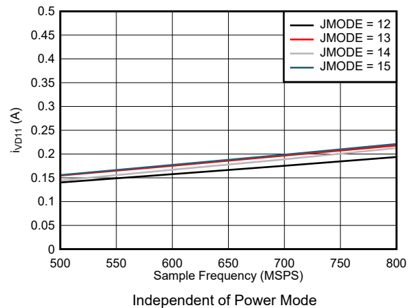
Figure 5-90. Dual Channel, I_{VD11} vs F_S for JMODES 12 - 15
