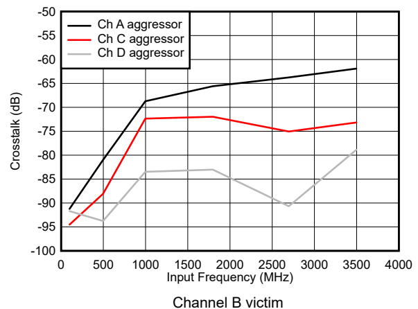
Figure 5-62. Crosstalk vs Input Frequency
