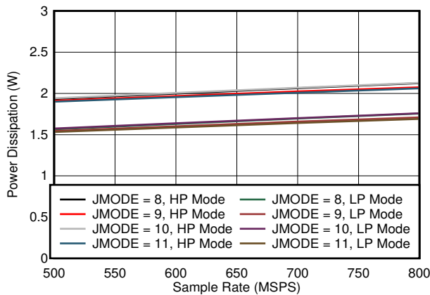
Figure 5-73. Quad Channel, Power Dissipation vs F_S for JMODES 8 - 11
