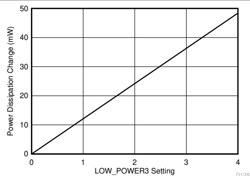
Figure 6-13. Power Dissipation Change vs LOW_POWER3 register setting
