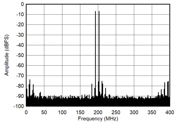
Figure 5-52. Dual Tone FFT at 998 MHz
