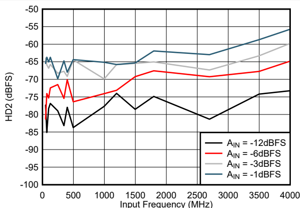
Figure 5-18. HD2 vs Input Frequency
