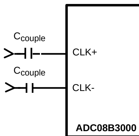
Figure 47. Differential Sample Clock Connection
