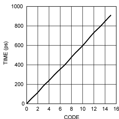
Figure 49. Typical Coarse Clock Phase Adjust Range
