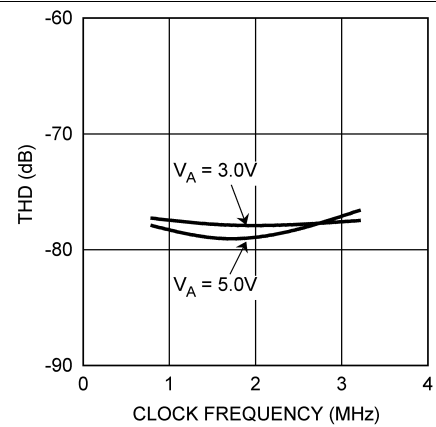
Figure 20. THD vs Clock Frequency
