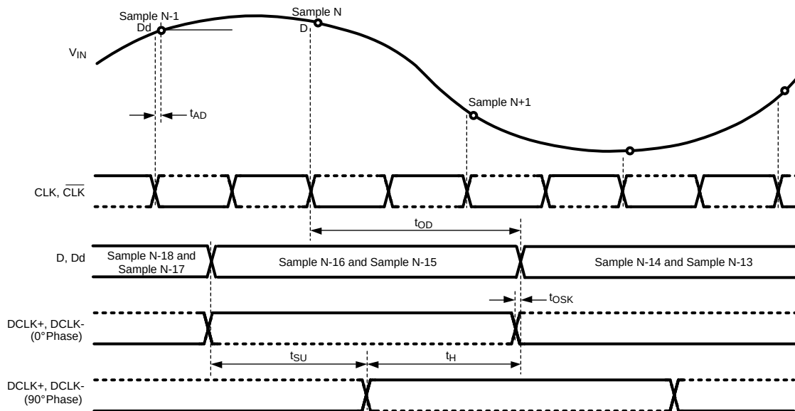
Figure 3. ADC081500 Timing — DDR Clocking
