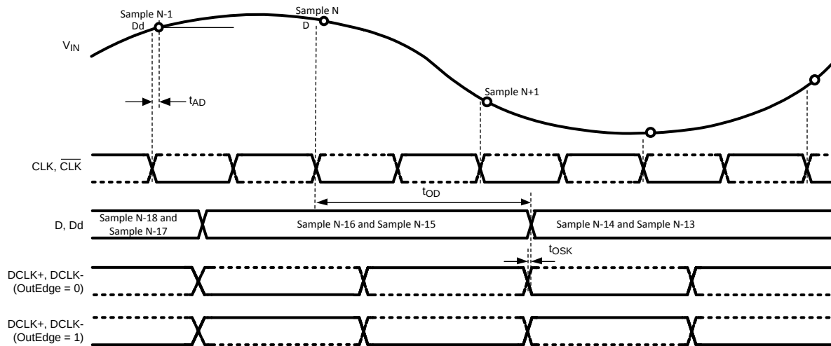
Figure 2. ADC081500 Timing — SDR Clocking
