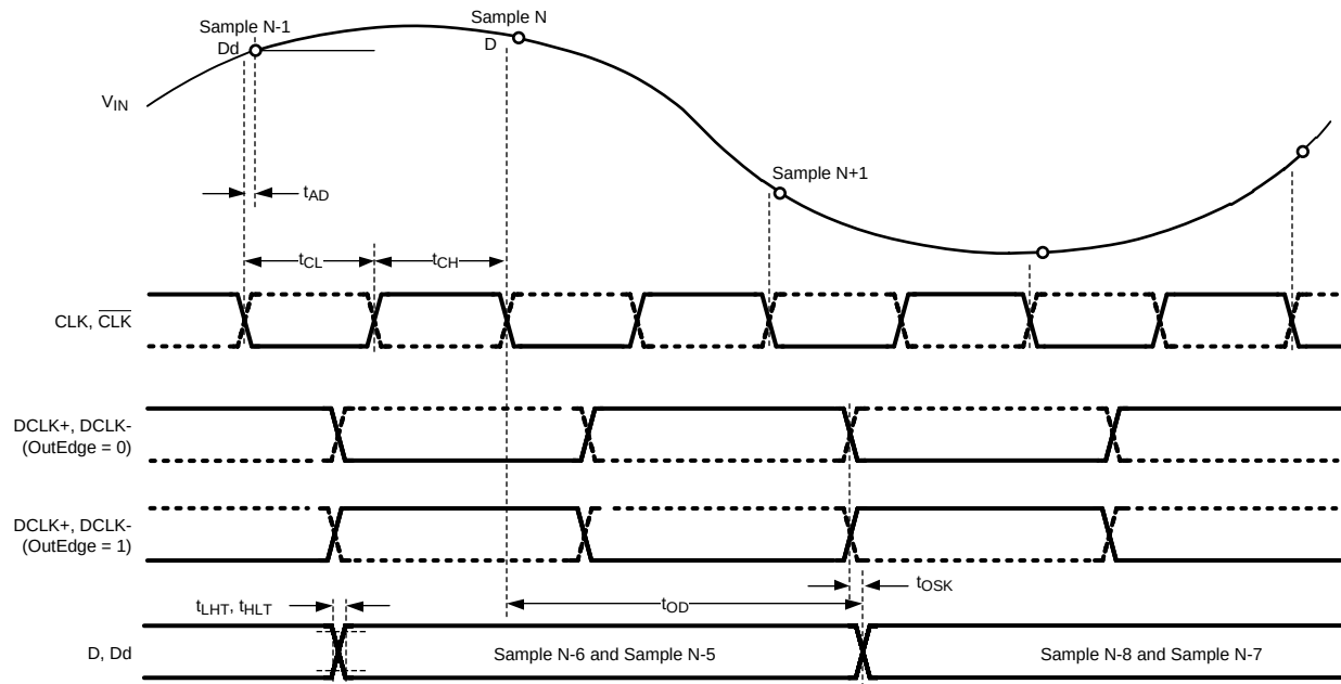
Figure 3. ADC081000 Timing
