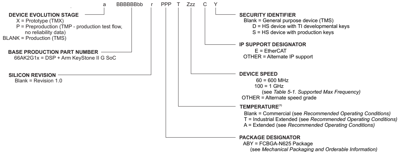
Figure 8-1. Device Nomenclature
