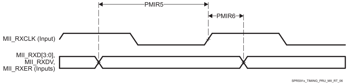
Figure 5-76. PRU-ICSS MII_RXD[3:0], MII_RXDV, and MII_RXER Timing
