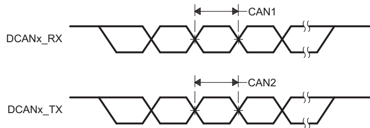
Figure 5-23. DCANx Timings
