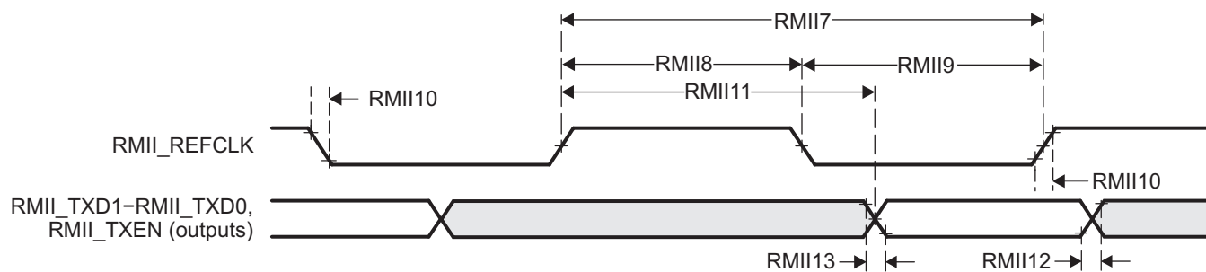
Figure 5-31. EMAC Transmit Interface Timing RMI Operation
