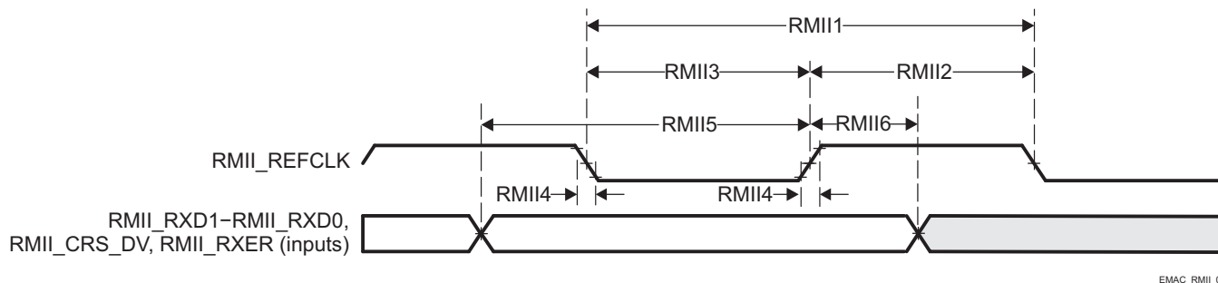
Figure 5-30. EMAC Receive Interface Timing RMI operation
