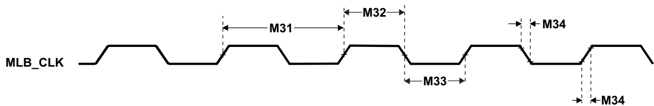
Figure 5-53. MLB_CLK Timing
