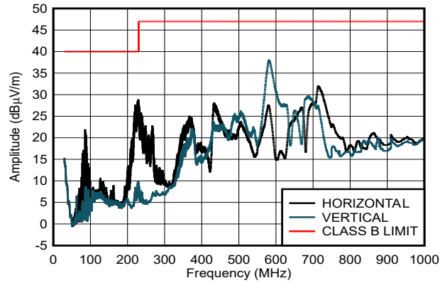
Figure 8-26. Radiated Emissions Test CISPR32 Class B Limits
