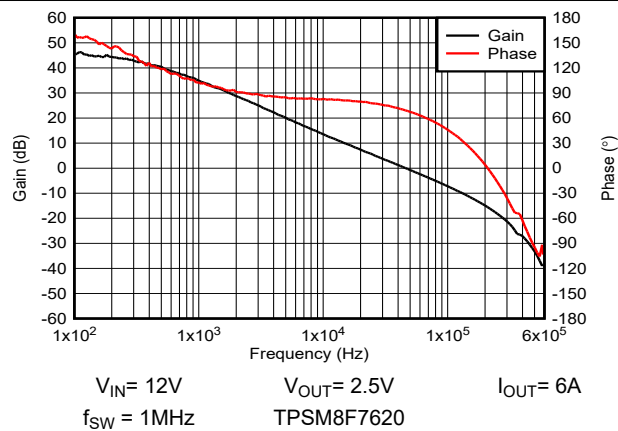
Figure 8-10. Voltage Loop Bode Plot VOUT3
