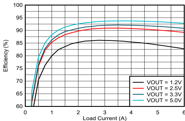
Typical Efficiency, 12V Input, 1MHz Fsw
