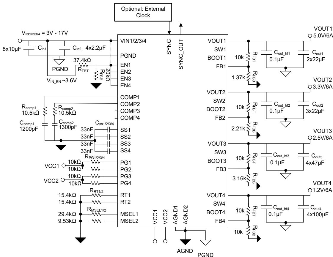
Figure 8-1. Four Output Application Schematic
