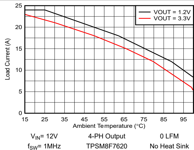
Figure 6-4. Maximum Output Current vs Ambient Temperature
