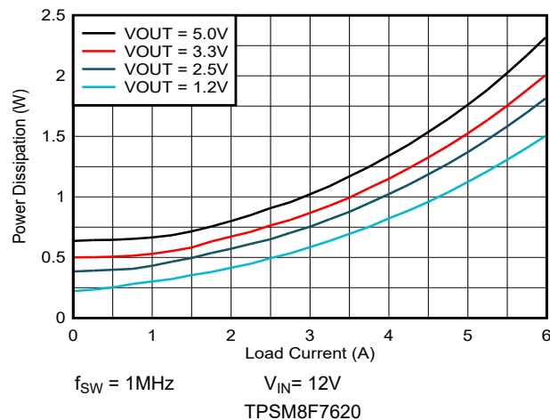
Figure 8-4. Power Dissipation
