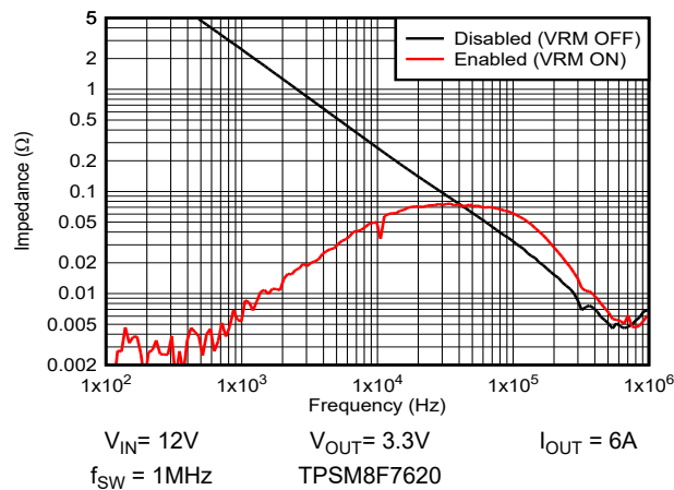
Figure 8-12. VOUT2 Output Impedance
