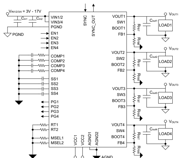
Typical Schematic
