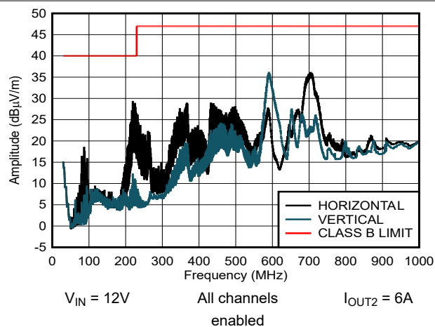
Figure 8-41. Radiated Emissions Test CISPR32 Class B Limits
