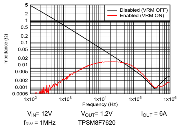
Figure 8-14. VOUT4 Output Impedance
