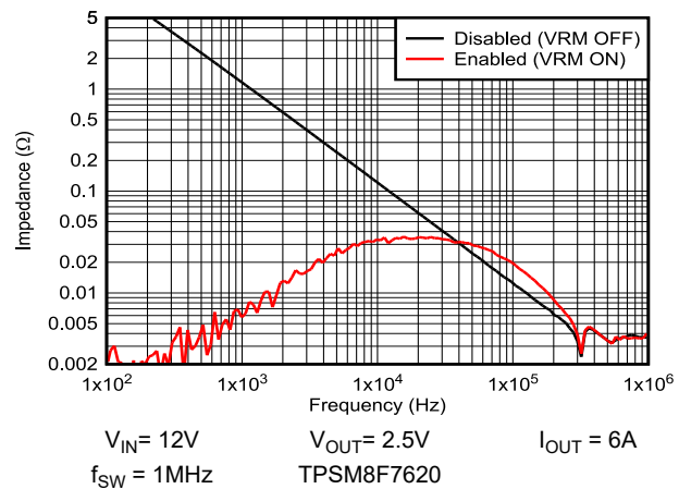
Figure 8-13. VOUT3 Output Impedance
