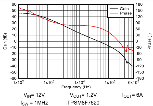
Figure 8-11. Voltage Loop Bode Plot VOUT4
