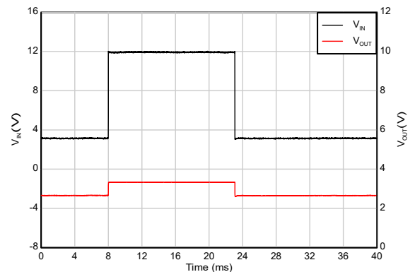
Figure 5-32. Line Transient
