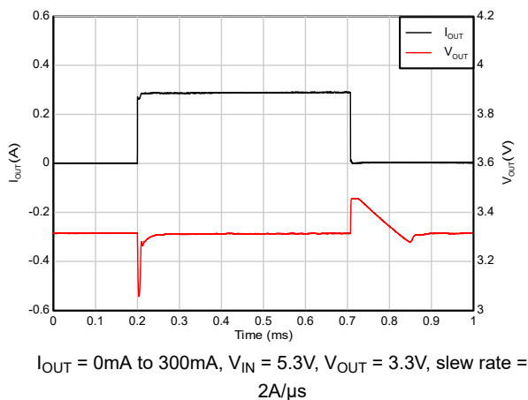
Figure 5-35. Load Transient
